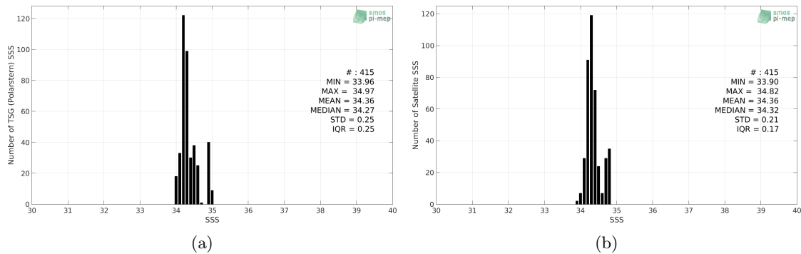
Figure 2: Histograms of SSS from TSG (Polarstern) (a) and CCI L4 Merged-OI v2.31 - 30-day running (ESA) (b) considering all match-up pairs per bins of 0.1 over the Pacific Ocean Pi-MEP region and for the full satellite product period.
