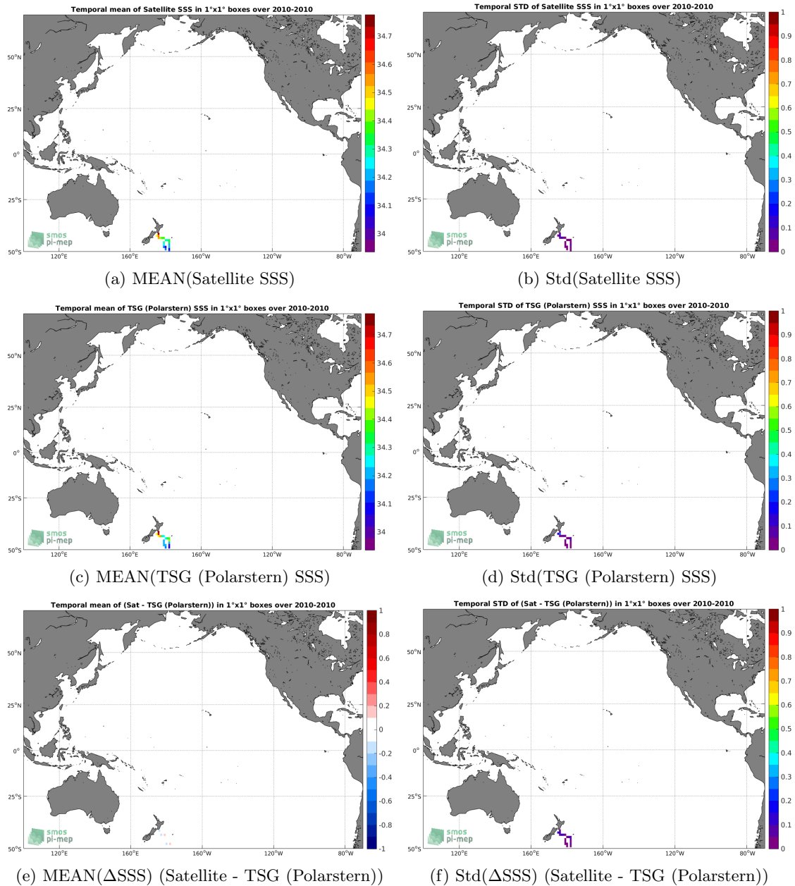
Figure 6: Temporal mean (left) and Std (right) of SSS from CCI L4 Merged-OI v2.31 - 30-day running (ESA) (top), TSG (Polarstern) (middle), and of \Delta SSS (Satellite - TSG (Polarstern)). Only match-up pairs are used to generate these maps.
