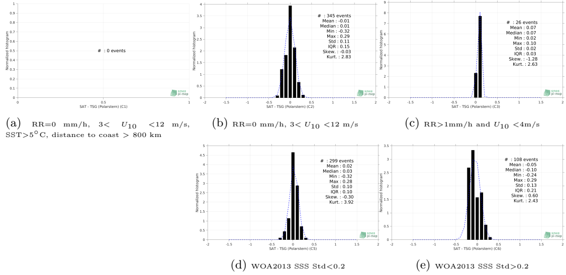
Figure 13: Normalized histogram of \Delta SSS (CCI L4 Merged-OI v2.31 - 30-day running (ESA) - TSG (Polarstern)) for 5 different subdatasets corresponding to: RR=0 mm/h, 3 < U_{10} < 12 m/s, SST>5°C, distance to coast > 800 km (a), RR=0 mm/h, 3 < U_{10} < 12 m/s (b), RR>1mm/h and U_{10} < 4 m/s (c), WOA2013 SSS Std<0.2 (d), WOA2013 SSS Std>0.2 (e).
