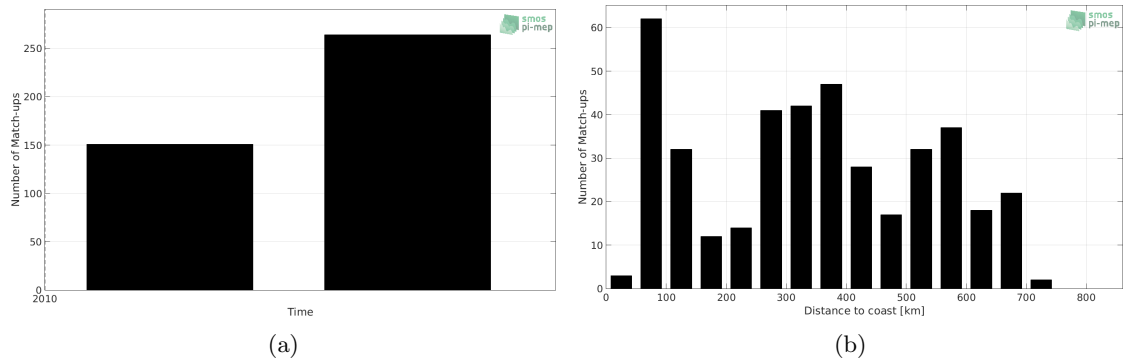
Figure 1: Number of match-ups between TSG (Polarstern) and CCI L4 Merged-OI v2.31 - 30-day running (ESA) SSS as a function of time (a) and as function of the distance to coast (b) over the Pacific Ocean Pi-MEP region and for the full satellite product period.
