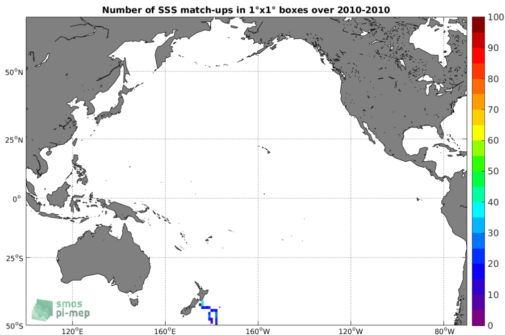
Figure 4: Number of SSS match-ups between TSG (Polarstern) SSS and the CCI L4 Merged-OI v2.31 - 30-day running (ESA) SSS product for the Pacific Ocean Pi-MEP region over 1^\circ \times 1^\circ boxes and for the full satellite product period.
