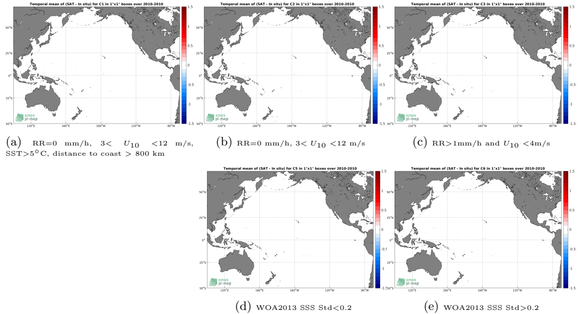
Figure 12: Temporal mean gridded over spatial boxes of size 1^{\circ}\times 1^{\circ} of \Delta\text{SSS} (CCI L4 Merged-OI v2.31 - 30-day running (ESA) - TSG (Polarstern)) for 5 different subdatasets corresponding to:RR=0 mm/h, 3 < U_{10} < 12 m/s, SST >5^{\circ}\text{C} , distance to coast > 800 km (a), RR=0 mm/h, 3 < U_{10} < 12 m/s (b), RR >1 mm/h and U_{10} < 4 m/s (c), WOA2013 SSS Std <0.2 (d), WOA2013 SSS Std >0.2 (e).
