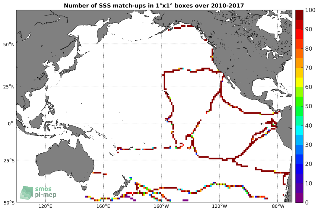
Figure 4: Number of SSS match-ups between TSG (GOSUD-Sailing-ship) SSS and the CCI L4 Merged-OI v2.31 - 30-day running (ESA) SSS product for the Pacific Ocean Pi-MEP region over 1^\circ \times 1^\circ boxes and for the full satellite product period.
