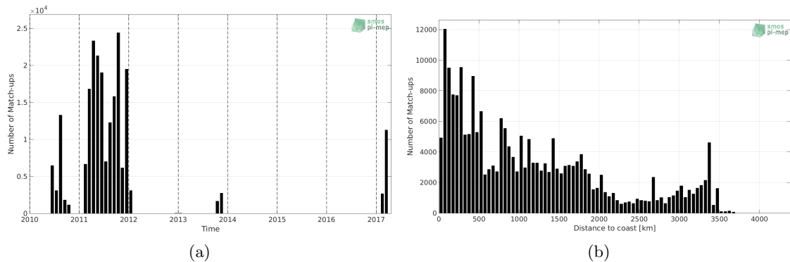
Figure 1: Number of match-ups between TSG (GOSUD-Sailing-ship) and CCI L4 Merged-OI v2.31 - 30-day running (ESA) SSS as a function of time (a) and as function of the distance to coast (b) over the Pacific Ocean Pi-MEP region and for the full satellite product period.
