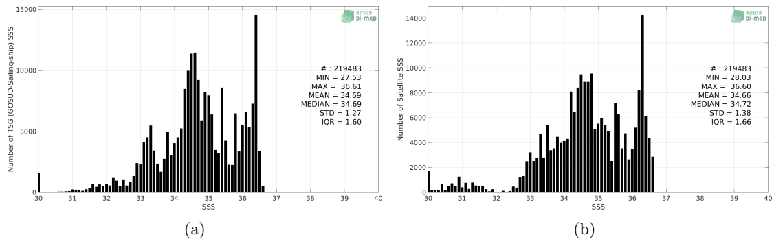
Figure 2: Histograms of SSS from TSG (GOSUD-Sailing-ship) (a) and CCI L4 Merged-OI v2.31 - 30-day running (ESA) (b) considering all match-up pairs per bins of 0.1 over the Pacific Ocean Pi-MEP region and for the full satellite product period.
