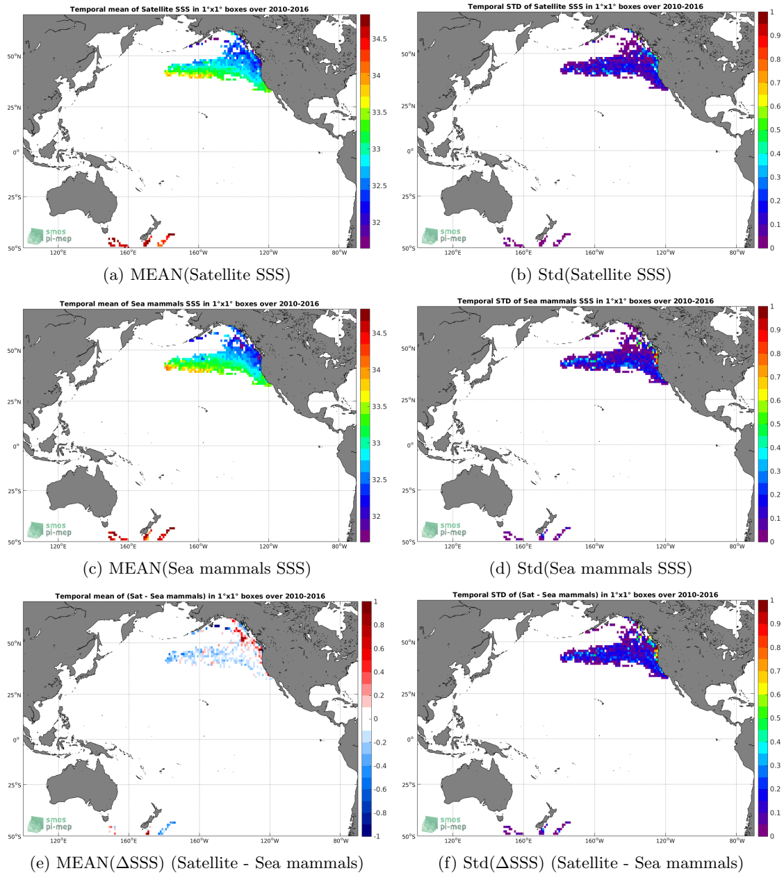
Figure 6: Temporal mean (left) and Std (right) of SSS from CCI L4 Merged-OI v2.31 - 30-day running (ESA) (top), Sea mammals (middle), and of \Delta SSS (Satellite - Sea mammals). Only match-up pairs are used to generate these maps.
