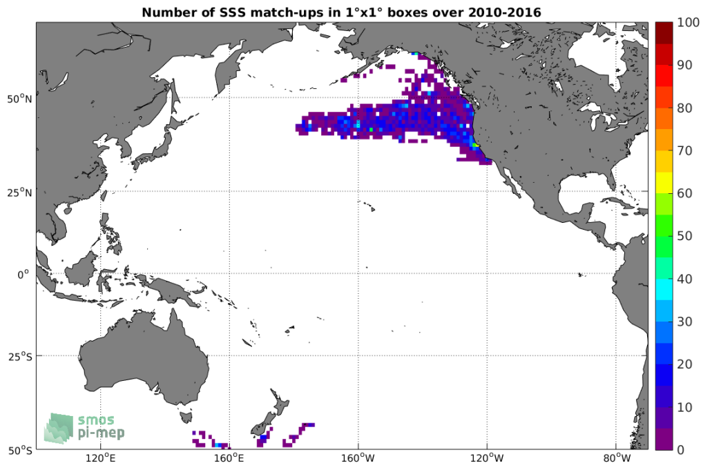
Figure 4: Number of SSS match-ups between Sea mammals SSS and the CCI L4 Merged-OI v2.31 - 30-day running (ESA) SSS product for the Pacific Ocean Pi-MEP region over 1°x1° boxes and for the full satellite product period.
