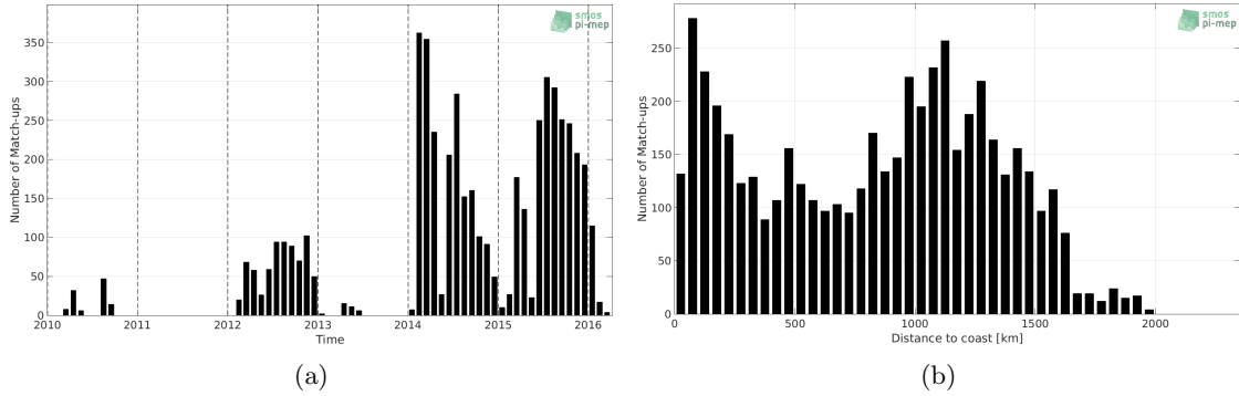
Figure 1: Number of match-ups between Sea mammals and CCI L4 Merged-OI v2.31 - 30-day running (ESA) SSS as a function of time (a) and as function of the distance to coast (b) over the Pacific Ocean Pi-MEP region and for the full satellite product period.
