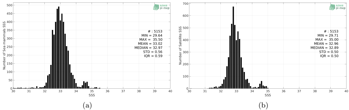
Figure 2: Histograms of SSS from Sea mammals (a) and CCI L4 Merged-OI v2.31 - 30-day running (ESA) (b) considering all match-up pairs per bins of 0.1 over the Pacific Ocean Pi-MEP region and for the full satellite product period.
