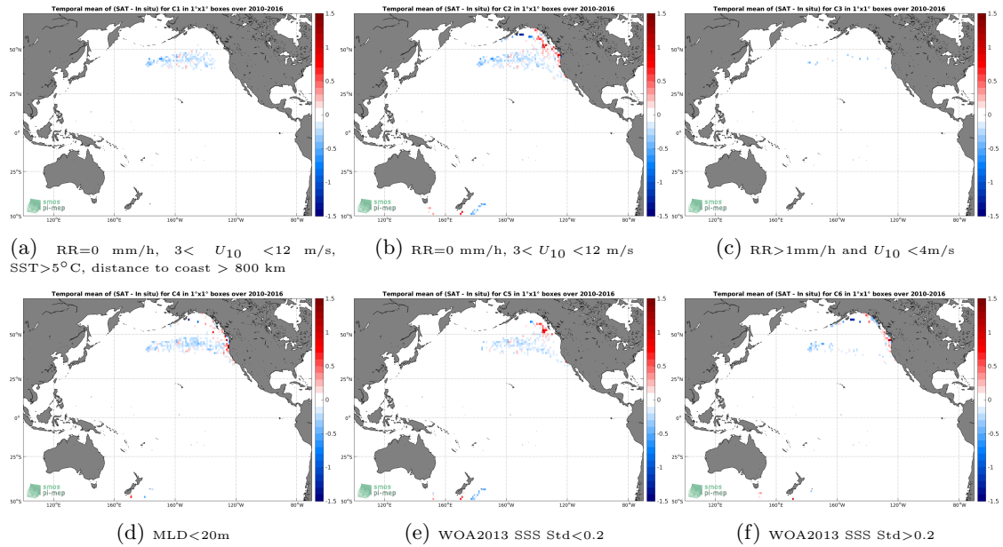
Figure 12: Temporal mean gridded over spatial boxes of size 1°x1° of \Delta SSS (CCI L4 Merged-OI v2.31 - 30-day running (ESA) - Sea mammals) for 6 different subdatasets corresponding to:RR=0 mm/h, 3 < U_{10} < 12 m/s, SST > 5°C, distance to coast > 800 km (a), RR=0 mm/h, 3 < U_{10} < 12 m/s (b), RR > 1mm/h and U_{10} < 4 m/s (c),MLD < 20m (d),WOA2013 SSS Std < 0.2 (e),WOA2013 SSS Std > 0.2 (f).
