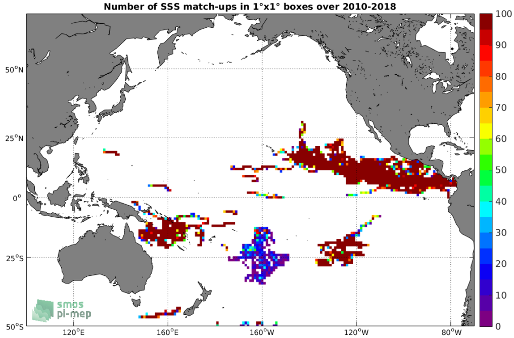
Figure 3: Number of SSS match-ups between Surface drifters SSS and the CCI SSS L4 Merged-OI v2.31 - 30-day running (ESA) SSS product for the Pacific Ocean Pi-MEP region over 1^\circ \times 1^\circ boxes and for the full satellite product period.
