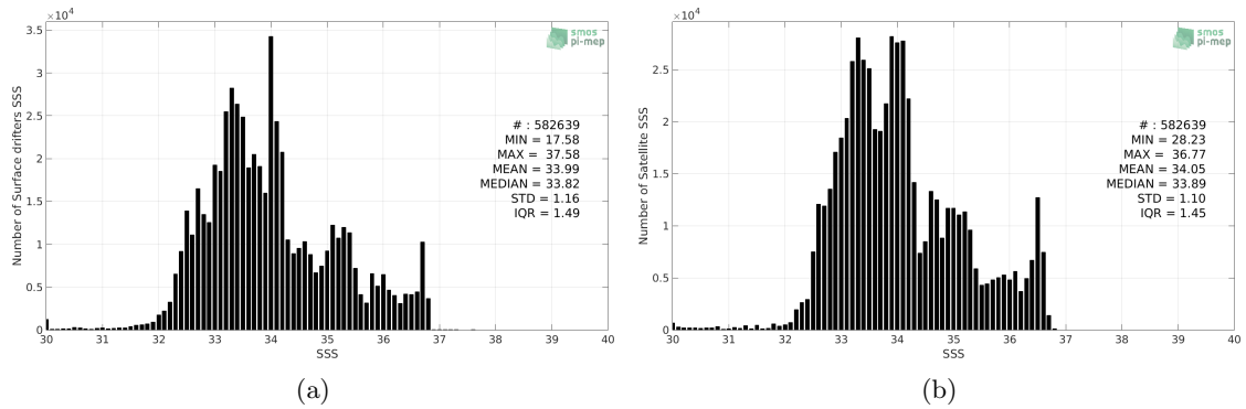
Figure 2: Histograms of SSS from Surface drifters (a) and CCI SSS L4 Merged-OI v2.31 - 30-day running (ESA) (b) considering all match-up pairs per bins of 0.1 over the Pacific Ocean Pi-MEP region and for the full satellite product period.
