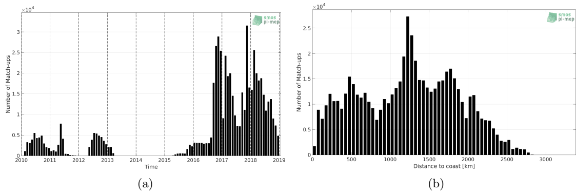
Figure 1: Number of match-ups between Surface drifters and CCI SSS L4 Merged-OI v2.31 - 30-day running (ESA) SSS as a function of time (a) and as function of the distance to coast (b) over the Pacific Ocean Pi-MEP region and for the full satellite product period.
