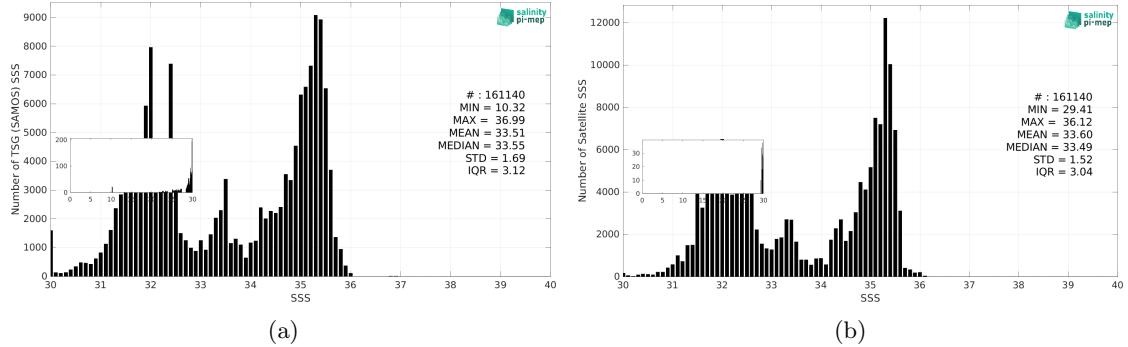
Figure 3: Histograms of SSS from TSG (SAMOS) (a) and Aquarius SSS L4 OI v5 - Weekly (IPRC) (b) considering all match-up pairs per bins of 0.1 over the Pacific Ocean Pi-MEP region and for the full satellite product period.
