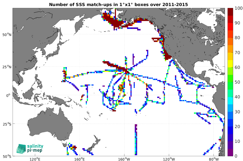
Figure 5: Number of SSS match-ups between TSG (SAMOS) SSS and the Aquarius SSS L4 OI v5 - Weekly (IPRC) SSS product for the Pacific Ocean Pi-MEP region over 1^\circ \times 1^\circ boxes and for the full satellite product period.
