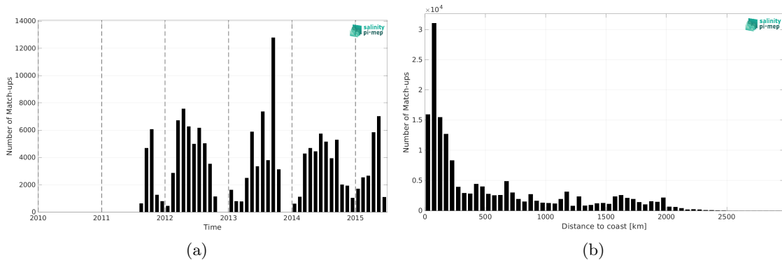
Figure 2: Number of match-ups between TSG (SAMOS) and Aquarius SSS L4 OI v5 - Weekly (IPRC) SSS as a function of time (a) and as function of the distance to coast (b) over the Pacific Ocean Pi-MEP region and for the full satellite product period.
