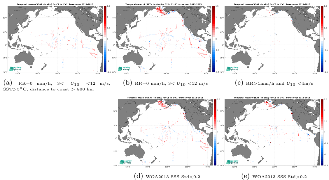
Figure 14: Temporal mean gridded over spatial boxes of size 1^\circ \times 1^\circ of \Delta SSS (Aquarius SSS L4 OI v5 - Weekly (IPRC) - TSG (SAMOS)) for 5 different subdatasets corresponding to: RR=0 mm/h, 3 < U_{10} < 12 m/s, SST > 5^\circ\text{C} , distance to coast > 800 km (a), RR=0 mm/h, 3 < U_{10} < 12 m/s (b), RR > 1 mm/h and U_{10} < 4 m/s (c), WOA2013 SSS Std < 0.2 (d), WOA2013 SSS Std > 0.2 (e).
