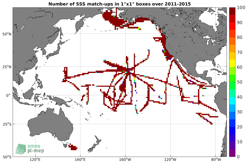
Figure 4: Number of SSS match-ups between TSG (SAMOS) SSS and the Aquarius SSS L4 OI v5 - Weekly (IPRC) SSS product for the Pacific Ocean Pi-MEP region over 1°x1° boxes and for the full satellite product period.
