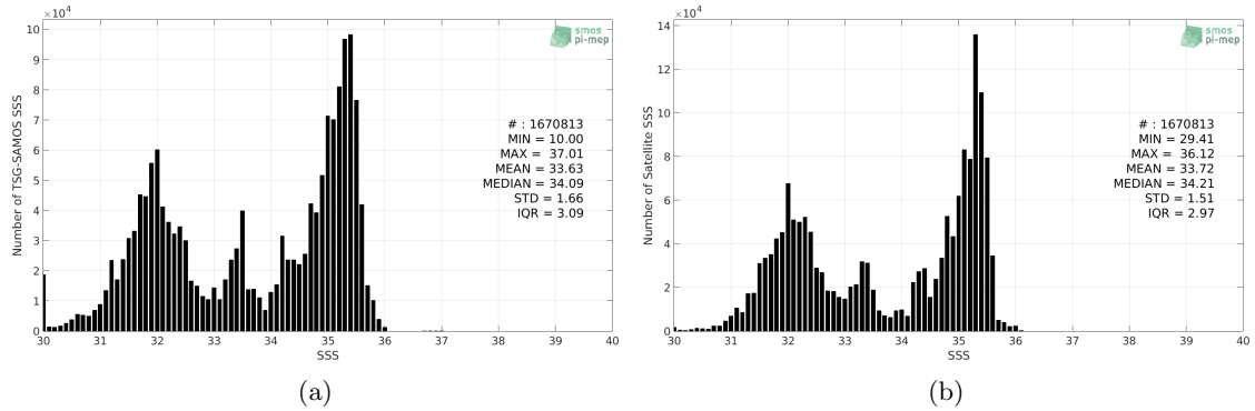
Figure 2: Histograms of SSS from TSG-SAMOS (a) and Aquarius-L4-IPRC-V5-WEEKLY (b) considering all match-up pairs per bins of 0.1 over the Pacific Ocean Pi-MEP region and for the full satellite product period.
