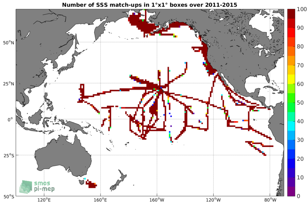
Figure 4: Number of SSS match-ups between TSG-SAMOS SSS and the Aquarius-L4-IPRC-V5-WEEKLY SSS product for the Pacific Ocean Pi-MEP region over 1°x1° boxes and for the full satellite product period.
