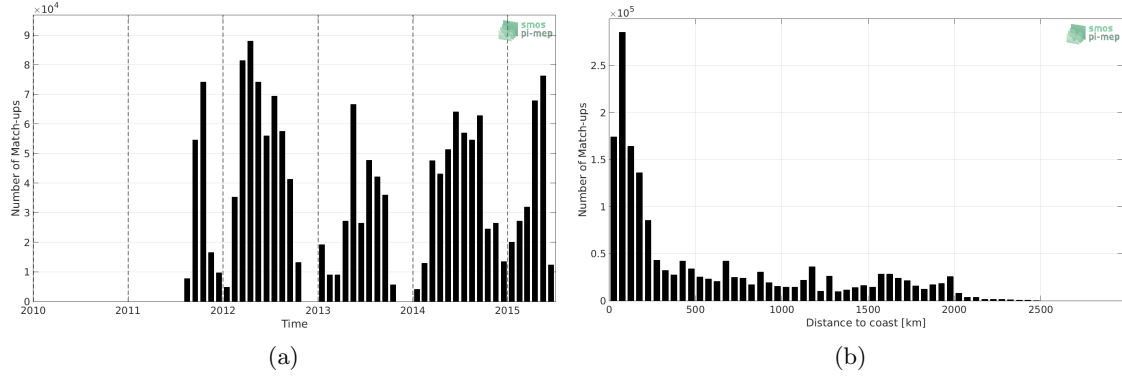
Figure 1: Number of match-ups between TSG-SAMOS and Aquarius-L4-IPRC-V5-WEEKLY SSS as a function of time (a) and as function of the distance to coast (b) over the Pacific Ocean Pi-MEP region and for the full satellite product period.
