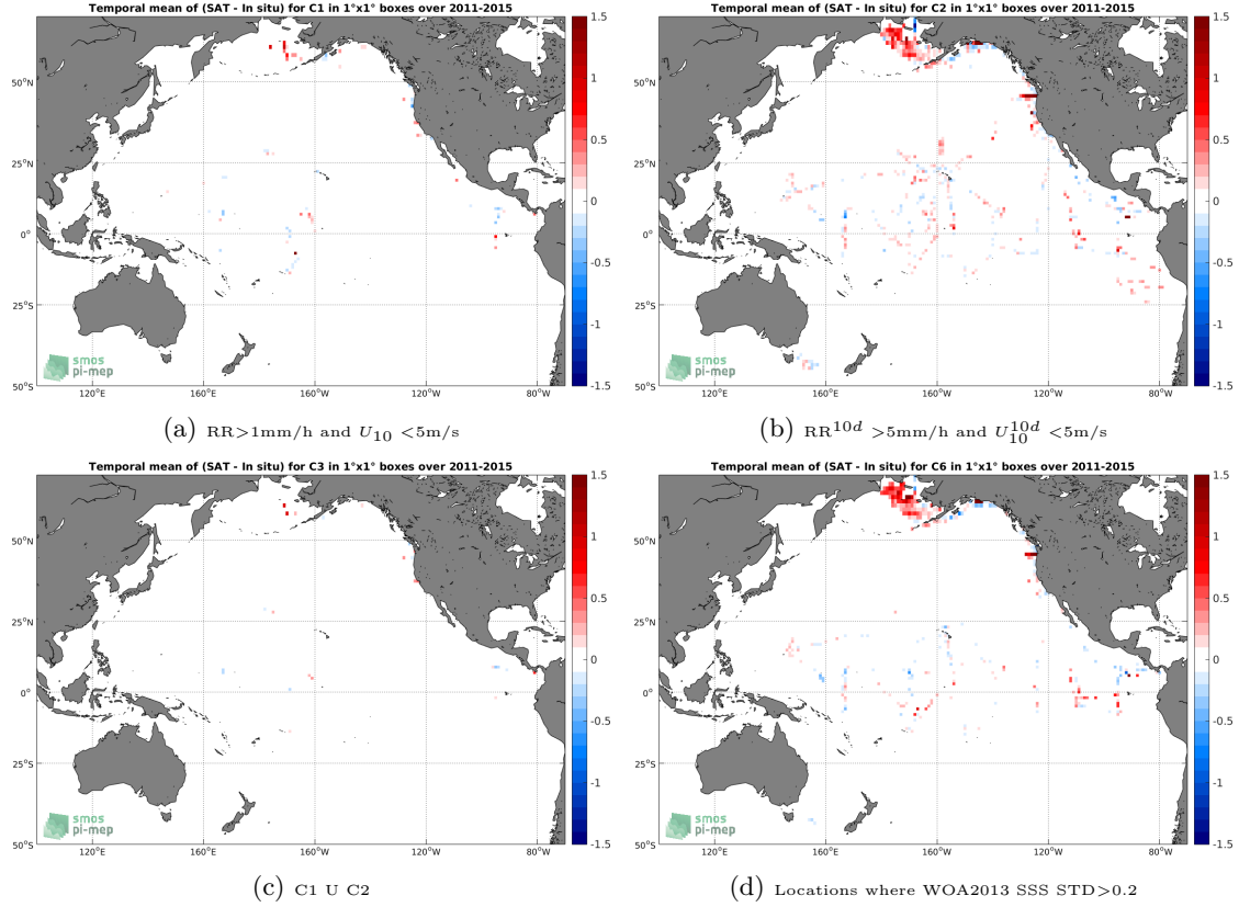
Figure 12: Temporal mean gridded over spatial boxes of size 1^\circ \times 1^\circ of \Delta SSS (Aquarius-L4-IPRC-V5-WEEKLY - TSG-SAMOS) for 4 different subdatasets corresponding to: RR > 1mm/h and U_{10} < 5\text{m/s} (a), RR 10d > 5mm/h and U_{10}^{10d} < 5\text{m/s} (b), C1 U C2 (c), Locations where WOA2013 SSS STD > 0.2 (d).
