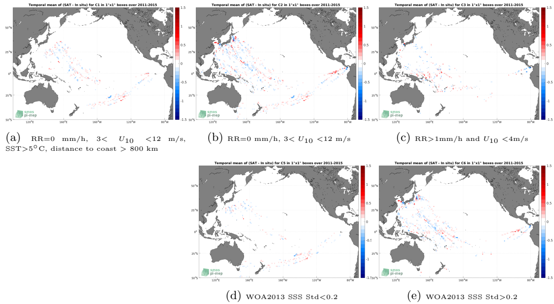
Figure 12: Temporal mean gridded over spatial boxes of size 1^\circ \times 1^\circ of \Delta SSS (Aquarius SSS L4 OI v5 - Weekly (IPRC) - TSG (LEGOS-DM)) for 5 different subdatasets corresponding to:RR=0 mm/h, 3 < U_{10} < 12 m/s, SST > 5^\circ\text{C} , distance to coast > 800 km (a), RR=0 mm/h, 3 < U_{10} < 12 m/s (b), RR > 1 mm/h and U_{10} < 4 m/s (c), WOA2013 SSS Std < 0.2 (d), WOA2013 SSS Std > 0.2 (e).
