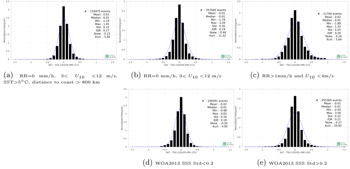
Figure 13: Normalized histogram of \Delta SSS (Aquarius SSS L4 OI v5 - Weekly (IPRC) - TSG (LEGOS-DM)) for 5 different subdatasets corresponding to: RR=0 mm/h, 3 < U_{10} < 12 m/s, SST > 5°C, distance to coast > 800 km (a), RR=0 mm/h, 3 < U_{10} < 12 m/s (b), RR > 1mm/h and U_{10} < 4 m/s (c), WOA2013 SSS Std < 0.2 (d), WOA2013 SSS Std > 0.2 (e).
