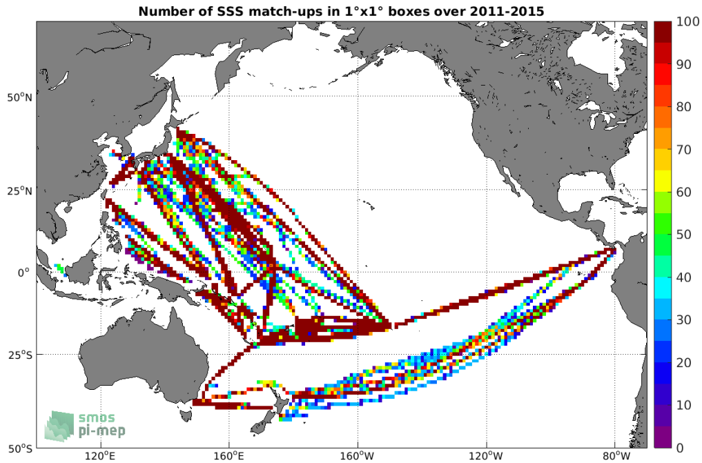
Figure 4: Number of SSS match-ups between TSG (LEGOS-DM) SSS and the Aquarius SSS L4 OI v5 - Weekly (IPRC) SSS product for the Pacific Ocean Pi-MEP region over 1°x1° boxes and for the full satellite product period.
