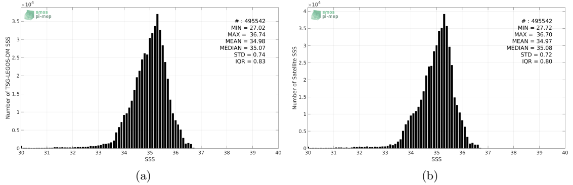
Figure 2: Histograms of SSS from TSG-LEGOS-DM (a) and Aquarius-L4-IPRC-V5-WEEKLY (b) considering all match-up pairs per bins of 0.1 over the Pacific Ocean Pi-MEP region and for the full satellite product period.
