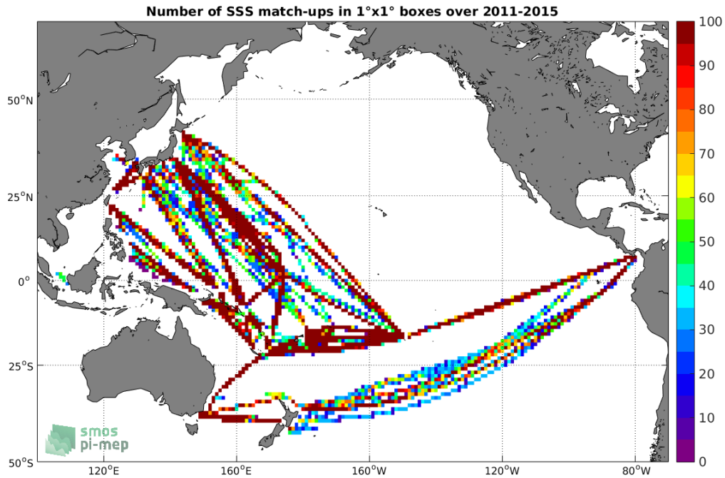
Figure 4: Number of SSS match-ups between TSG-LEGOS-DM SSS and the Aquarius-L4-IPRC-V5-WEEKLY SSS product for the Pacific Ocean Pi-MEP region over 1^\circ \times 1^\circ boxes and for the full satellite product period.
