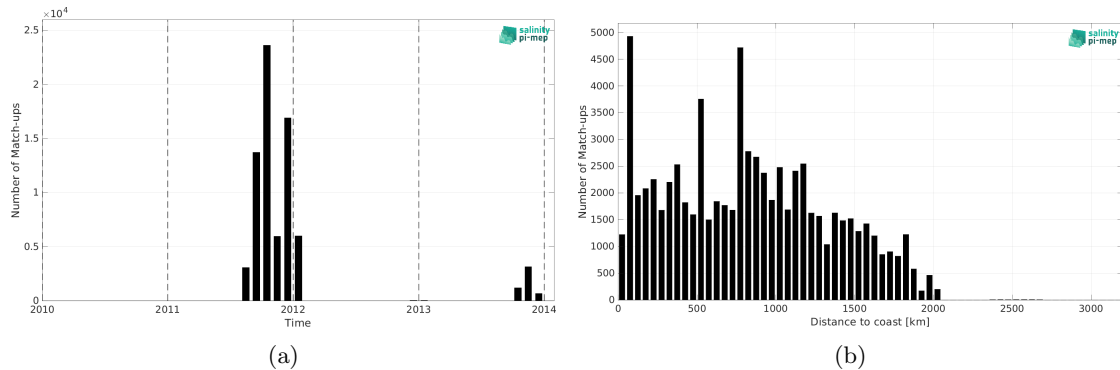
Figure 2: Number of match-ups between TSG (GOSUD-Sailing-ship) and Aquarius SSS L4 OI v5 - Weekly (IPRC) SSS as a function of time (a) and as function of the distance to coast (b) over the Pacific Ocean Pi-MEP region and for the full satellite product period.
