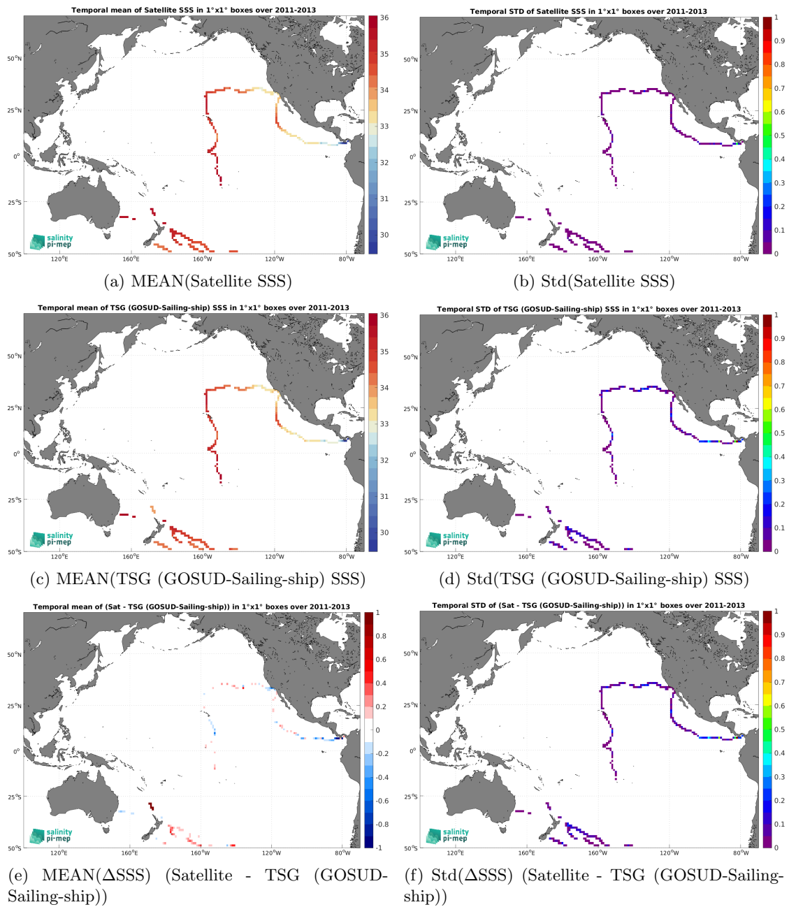
Figure 7: Temporal mean (left) and Std (right) of SSS from Aquarius SSS L4 OI v5 - Weekly (IPRC) (top), TSG (GOSUD-Sailing-ship) (middle), and of \Delta SSS (Satellite - TSG (GOSUD-Sailing-ship)). Only match-up pairs are used to generate these maps.
