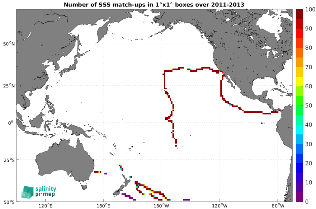
Figure 5: Number of SSS match-ups between TSG (GOSUD-Sailing-ship) SSS and the Aquarius SSS L4 OI v5 - Weekly (IPRC) SSS product for the Pacific Ocean Pi-MEP region over 1^\circ \times 1^\circ boxes and for the full satellite product period.
