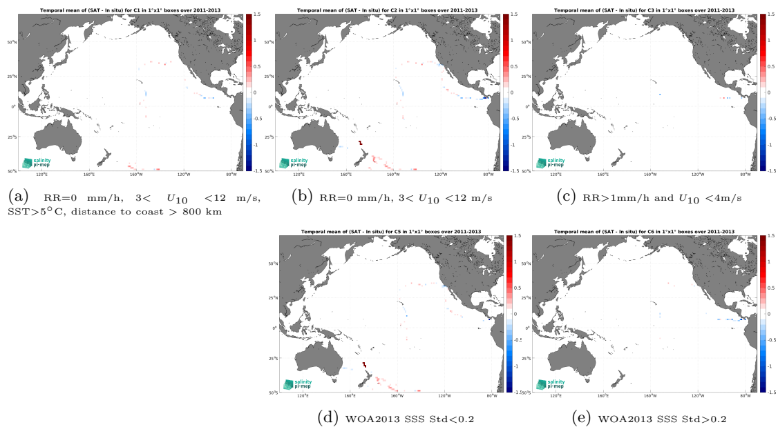
Figure 14: Temporal mean gridded over spatial boxes of size 1^\circ \times 1^\circ of \Delta SSS (Aquarius SSS L4 OI v5 - Weekly (IPRC) - TSG (GOSUD-Sailing-ship)) for 5 different subdatasets corresponding to: RR=0 mm/h, 3 < U_{10} < 12 m/s, SST > 5^\circ\text{C} , distance to coast > 800 km (a), RR=0 mm/h, 3 < U_{10} < 12 m/s (b), RR > 1 mm/h and U_{10} < 4 m/s (c), WOA2013 SSS Std < 0.2 (d), WOA2013 SSS Std > 0.2 (e).
