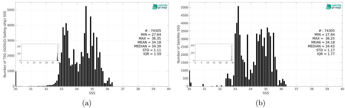
Figure 3: Histograms of SSS from TSG (GOSUD-Sailing-ship) (a) and Aquarius SSS L4 OI v5 - Weekly (IPRC) (b) considering all match-up pairs per bins of 0.1 over the Pacific Ocean Pi-MEP region and for the full satellite product period.
