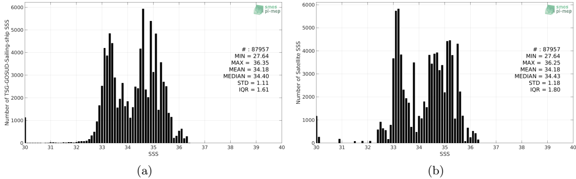
Figure 2: Histograms of SSS from TSG-GOSUD-Sailing-ship (a) and Aquarius-L4-IPRC-V5-WEEKLY (b) considering all match-up pairs per bins of 0.1 over the Pacific Ocean Pi-MEP region and for the full satellite product period.
