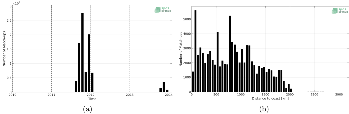
Figure 1: Number of match-ups between TSG-GOSUD-Sailing-ship and Aquarius-L4-IPRC-V5-WEEKLY SSS as a function of time (a) and as function of the distance to coast (b) over the Pacific Ocean Pi-MEP region and for the full satellite product period.
