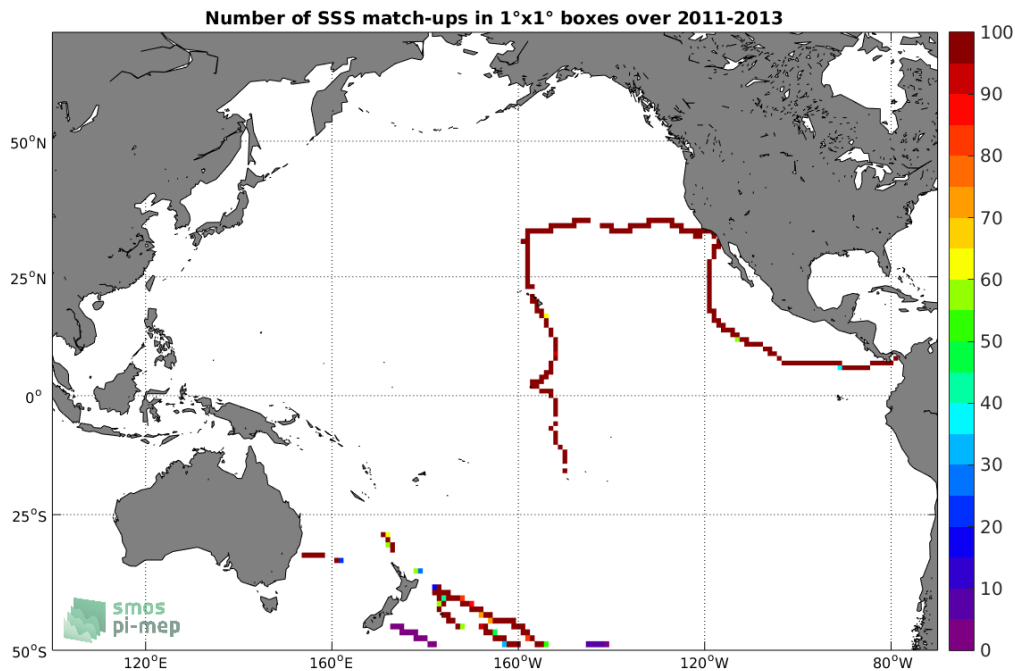
Figure 4: Number of SSS match-ups between TSG-GOSUD-Sailing-ship SSS and the Aquarius-L4-IPRC-V5-WEEKLY SSS product for the Pacific Ocean Pi-MEP region over 1^\circ \times 1^\circ boxes and for the full satellite product period.
