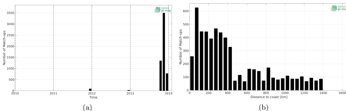
Figure 1: Number of match-ups between TSG-GOSUD-Sailing-ship and Aquarius-L4-IPRC-V5-WEEKLY SSS as a function of time (a) and as function of the distance to coast (b) over the Pacific Ocean Pi-MEP region and for the full satellite product period.
