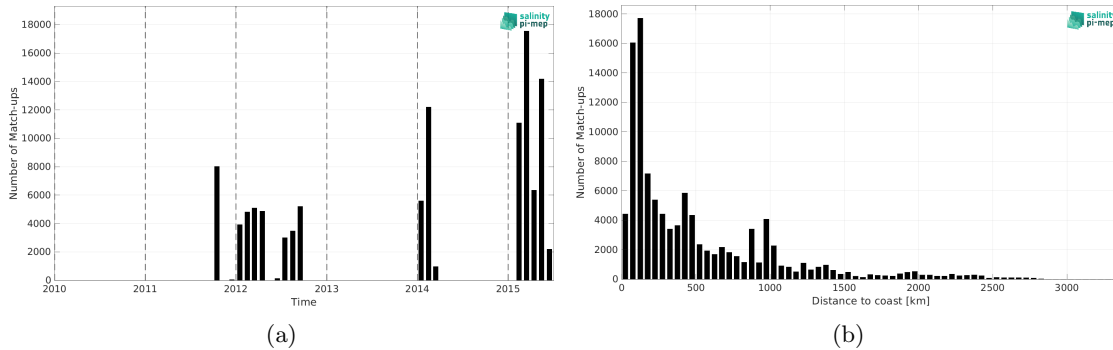
Figure 2: Number of match-ups between TSG (GOSUD-Research-vessel) and Aquarius SSS L4 OI v5 - Weekly (IPRC) SSS as a function of time (a) and as function of the distance to coast (b) over the Pacific Ocean Pi-MEP region and for the full satellite product period.
