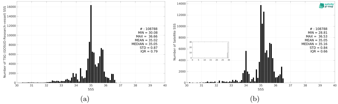
Figure 3: Histograms of SSS from TSG (GOSUD-Research-vessel) (a) and Aquarius SSS L4 OI v5 - Weekly (IPRC) (b) considering all match-up pairs per bins of 0.1 over the Pacific Ocean Pi-MEP region and for the full satellite product period.
