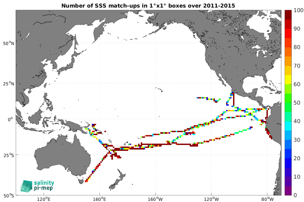
Figure 5: Number of SSS match-ups between TSG (GOSUD-Research-vessel) SSS and the Aquarius SSS L4 OI v5 - Weekly (IPRC) SSS product for the Pacific Ocean Pi-MEP region over 1^\circ \times 1^\circ boxes and for the full satellite product period.
