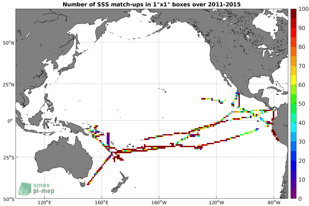
Figure 4: Number of SSS match-ups between TSG (GOSUD-Research-vessel) SSS and the Aquarius SSS L4 OI v5 - Weekly (IPRC) SSS product for the Pacific Ocean Pi-MEP region over 1°x1° boxes and for the full satellite product period.
