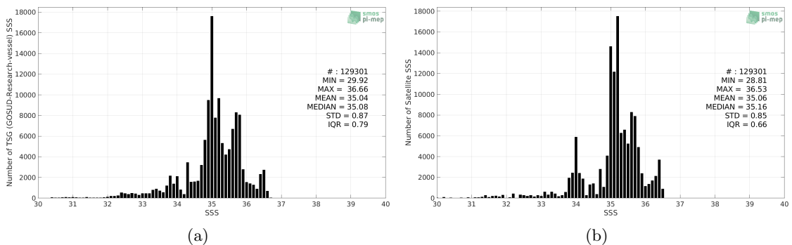
Figure 2: Histograms of SSS from TSG (GOSUD-Research-vessel) (a) and Aquarius SSS L4 OI v5 - Weekly (IPRC) (b) considering all match-up pairs per bins of 0.1 over the Pacific Ocean Pi-MEP region and for the full satellite product period.
