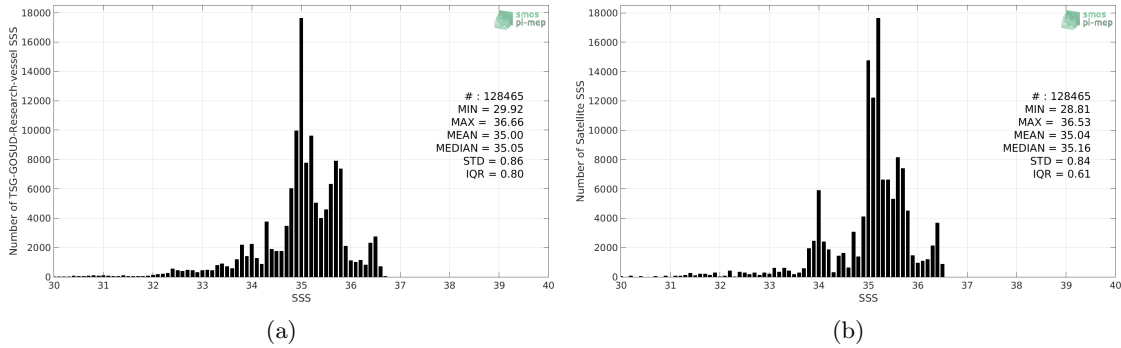
Figure 2: Histograms of SSS from TSG-GOSUD-Research-vessel (a) and Aquarius-L4-IPRC-V5-WEEKLY (b) considering all match-up pairs per bins of 0.1 over the Pacific Ocean Pi-MEP region and for the full satellite product period.
