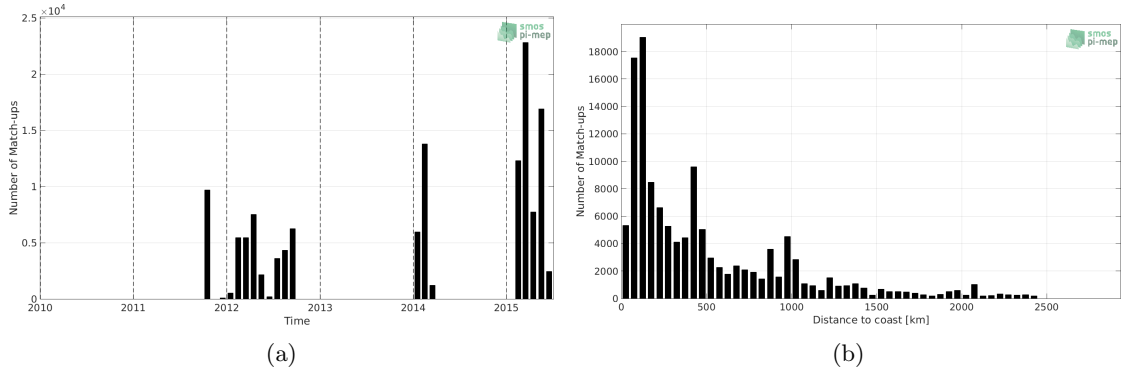
Figure 1: Number of match-ups between TSG-GOSUD-Research-vessel and Aquarius-L4-IPRC-V5-WEEKLY SSS as a function of time (a) and as function of the distance to coast (b) over the Pacific Ocean Pi-MEP region and for the full satellite product period.
