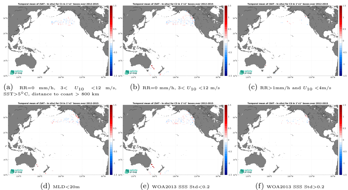
Figure 14: Temporal mean gridded over spatial boxes of size 1^\circ \times 1^\circ of \Delta SSS (Aquarius SSS L4 OI v5 - Weekly (IPRC) - Marine mammals) for 6 different subdatasets corresponding to:RR=0 mm/h, 3 < U_{10} < 12 m/s, SST>5°C, distance to coast > 800 km (a), RR=0 mm/h, 3 < U_{10} < 12 m/s (b), RR>1mm/h and U_{10} < 4 m/s (c),MLD<20m (d),WOA2013 SSS Std<0.2 (e),WOA2013 SSS Std>0.2 (f).
