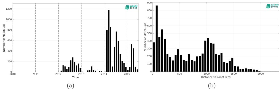
Figure 2: Number of match-ups between Marine mammals and Aquarius SSS L4 OI v5 - Weekly (IPRC) SSS as a function of time (a) and as function of the distance to coast (b) over the Pacific Ocean Pi-MEP region and for the full satellite product period.
