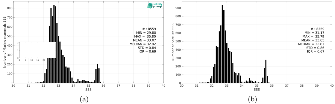
Figure 3: Histograms of SSS from Marine mammals (a) and Aquarius SSS L4 OI v5 - Weekly (IPRC) (b) considering all match-up pairs per bins of 0.1 over the Pacific Ocean Pi-MEP region and for the full satellite product period.
