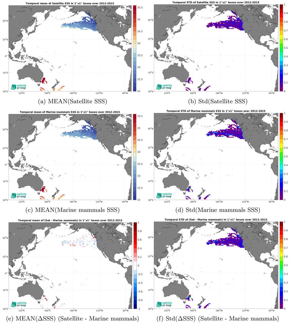
Figure 7: Temporal mean (left) and Std (right) of SSS from Aquarius SSS L4 OI v5 - Weekly (IPRC) (top), Marine mammals (middle), and of \Delta SSS (Satellite - Marine mammals). Only match-up pairs are used to generate these maps.
