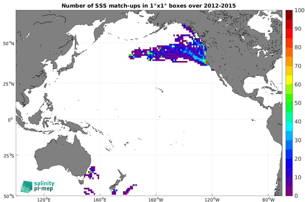
Figure 5: Number of SSS match-ups between Marine mammals SSS and the Aquarius SSS L4 OI v5 - Weekly (IPRC) SSS product for the Pacific Ocean Pi-MEP region over 1^\circ \times 1^\circ boxes and for the full satellite product period.
