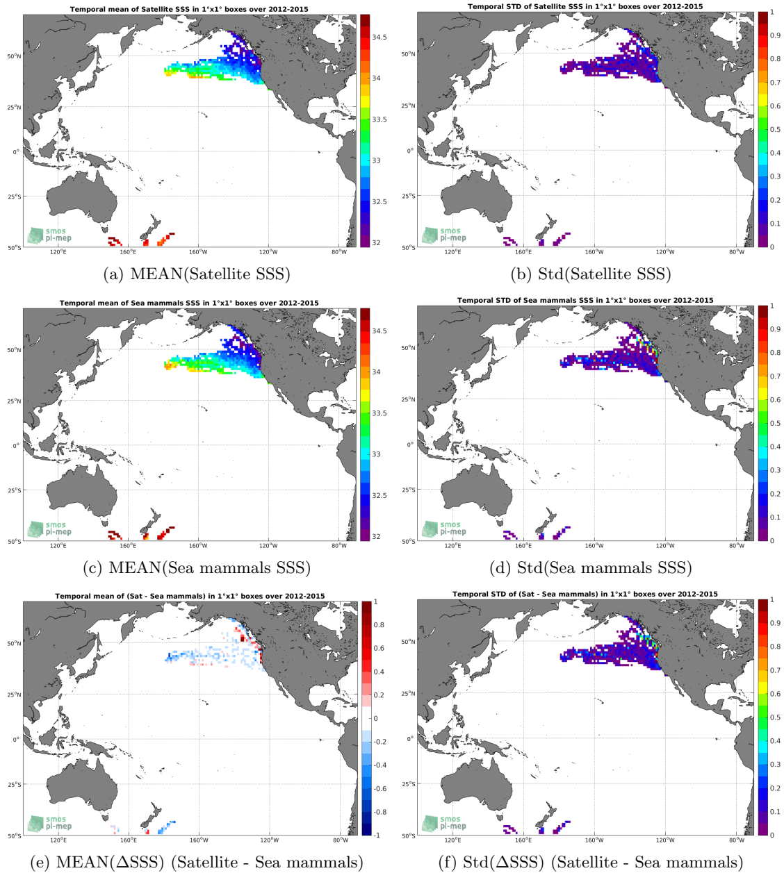
Figure 6: Temporal mean (left) and Std (right) of SSS from Aquarius-L4-IPRC-V5-WEEKLY (top), Sea mammals (middle), and of \Delta SSS (Satellite - Sea mammals). Only match-up pairs are used to generate these maps.
