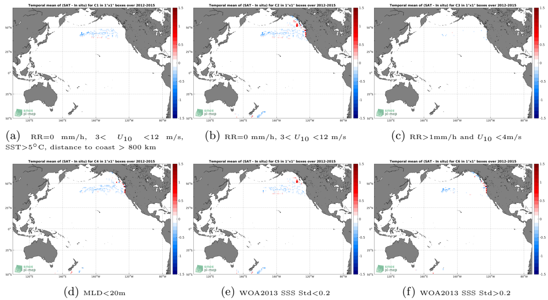
Figure 12: Temporal mean gridded over spatial boxes of size 1^\circ \times 1^\circ of \Delta SSS (Aquarius-L4-IPRC-V5-WEEKLY - Sea mammals) for 6 different subdatasets corresponding to:RR=0 mm/h, 3 < U_{10} < 12 m/s, SST >5^\circ C, distance to coast > 800 km (a), RR=0 mm/h, 3 < U_{10} < 12 m/s (b), RR >1 mm/h and U_{10} < 4 m/s (c),MLD <20 m (d),WOA2013 SSS Std <0.2 (e),WOA2013 SSS Std >0.2 (f).
