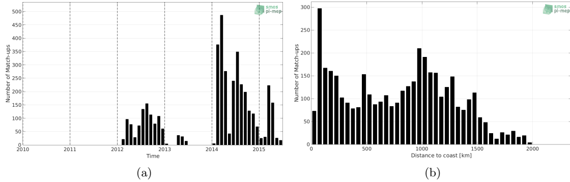
Figure 1: Number of match-ups between Sea mammals and Aquarius-L4-IPRC-V5-WEEKLY SSS as a function of time (a) and as function of the distance to coast (b) over the Pacific Ocean Pi-MEP region and for the full satellite product period.
