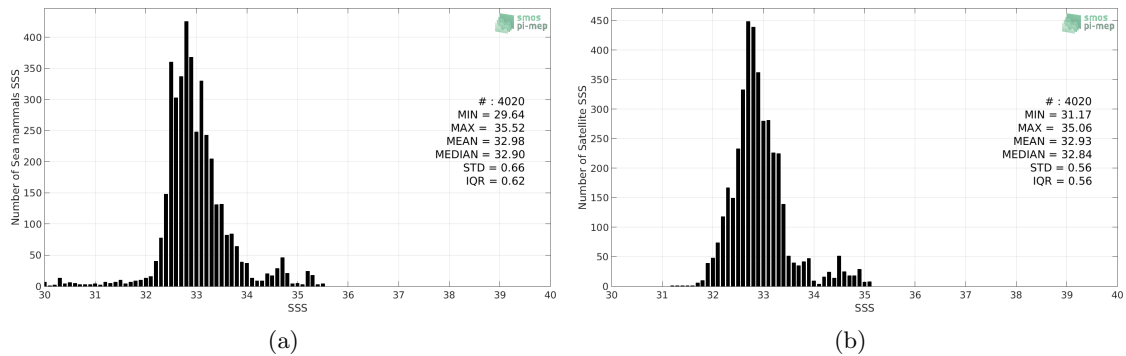
Figure 2: Histograms of SSS from Sea mammals (a) and Aquarius-L4-IPRC-V5-WEEKLY (b) considering all match-up pairs per bins of 0.1 over the Pacific Ocean Pi-MEP region and for the full satellite product period.
