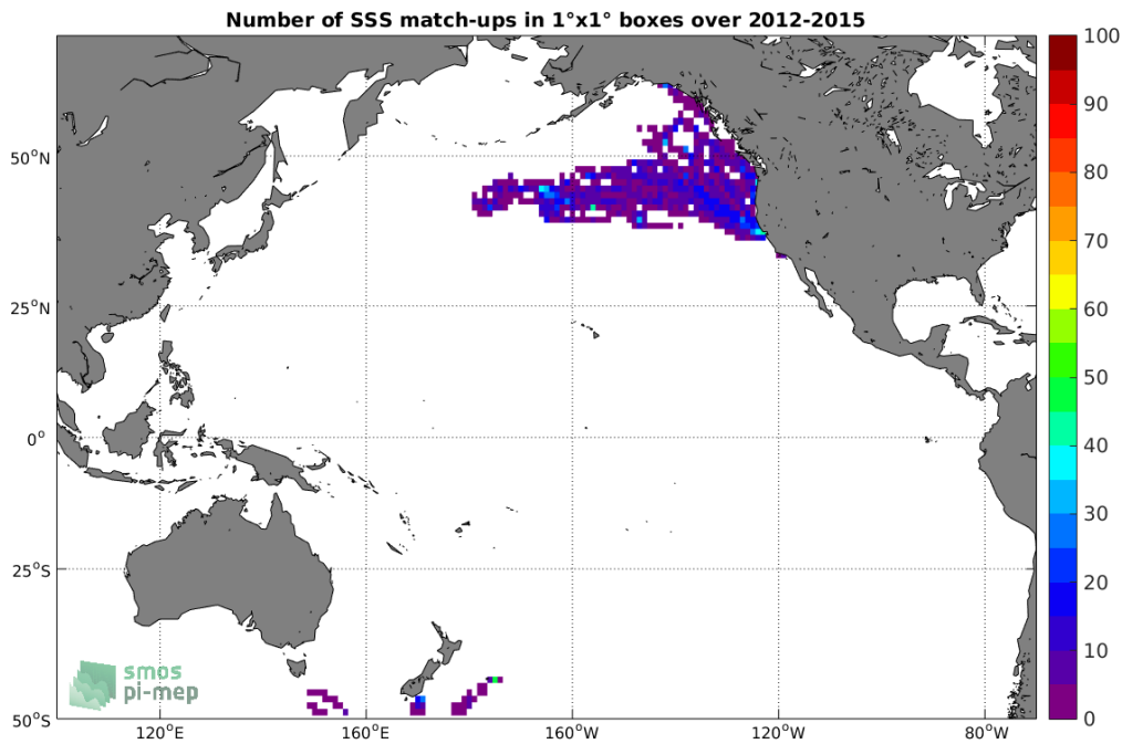
Figure 4: Number of SSS match-ups between Sea mammals SSS and the Aquarius-L4-IPRC-V5-WEEKLY SSS product for the Pacific Ocean Pi-MEP region over 1°x1° boxes and for the full satellite product period.
