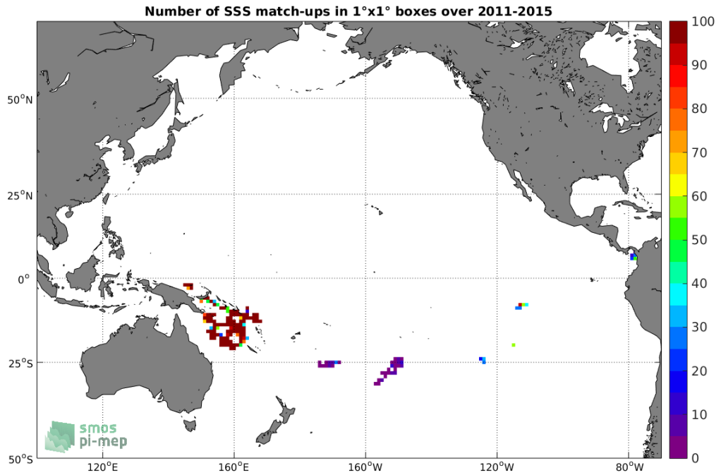
Figure 3: Number of SSS match-ups between Surface drifters SSS and the Aquarius-L4-IPRC-V5-WEEKLY SSS product for the Pacific Ocean Pi-MEP region over 1°x1° boxes and for the full satellite product period.
