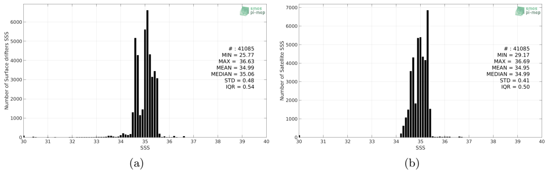
Figure 2: Histograms of SSS from Surface drifters (a) and Aquarius-L4-IPRC-V5-WEEKLY (b) considering all match-up pairs per bins of 0.1 over the Pacific Ocean Pi-MEP region and for the full satellite product period.
