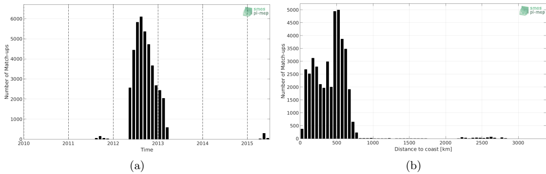
Figure 1: Number of match-ups between Surface drifters and Aquarius-L4-IPRC-V5-WEEKLY SSS as a function of time (a) and as function of the distance to coast (b) over the Pacific Ocean Pi-MEP region and for the full satellite product period.
