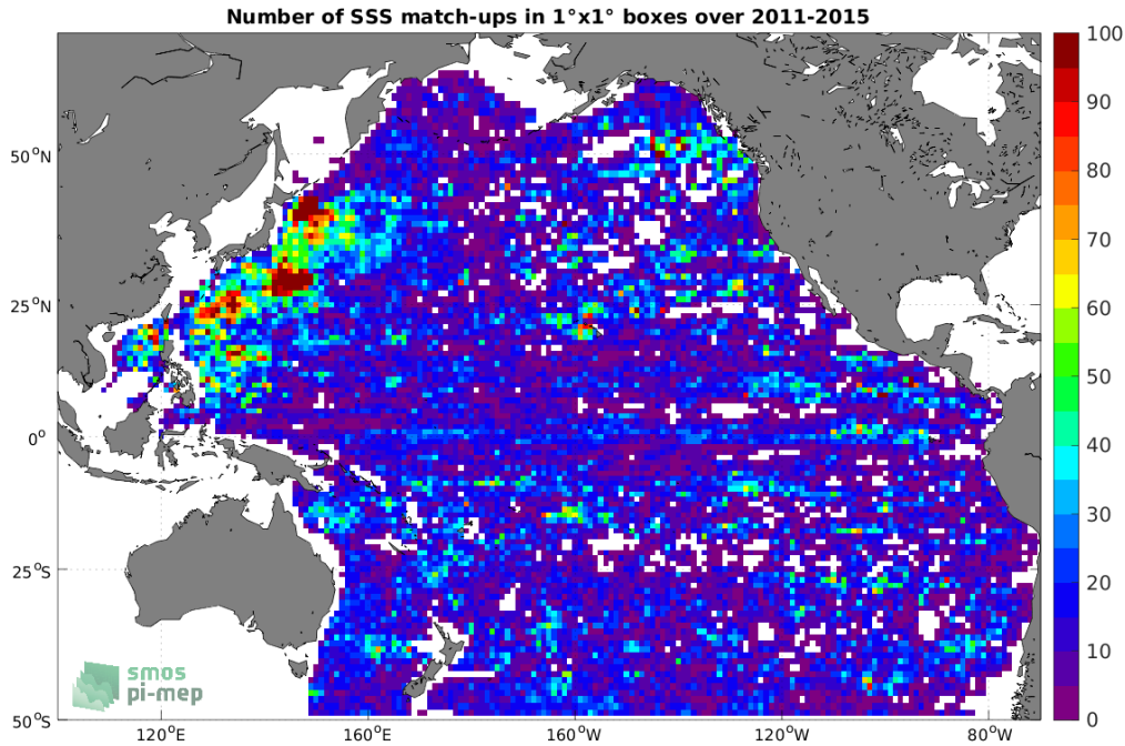
Figure 4: Number of SSS match-ups between Argo SSS and the Aquarius SSS L4 OI v5 - Weekly (IPRC) SSS product for the Pacific Ocean Pi-MEP region over 1^\circ \times 1^\circ boxes and for the full satellite product period.
