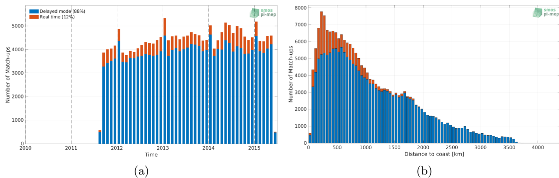
Figure 1: Number of match-ups between Argo and Aquarius SSS L4 OI v5 - Weekly (IPRC) SSS as a function of time (a) and as function of the distance to coast (b) over the Pacific Ocean Pi-MEP region and for the full satellite product period.
