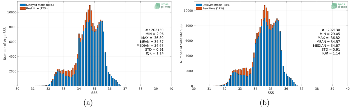
Figure 2: Histograms of SSS from Argo (a) and Aquarius SSS L4 OI v5 - Weekly (IPRC) (b) considering all match-up pairs per bins of 0.1 over the Pacific Ocean Pi-MEP region and for the full satellite product period.
