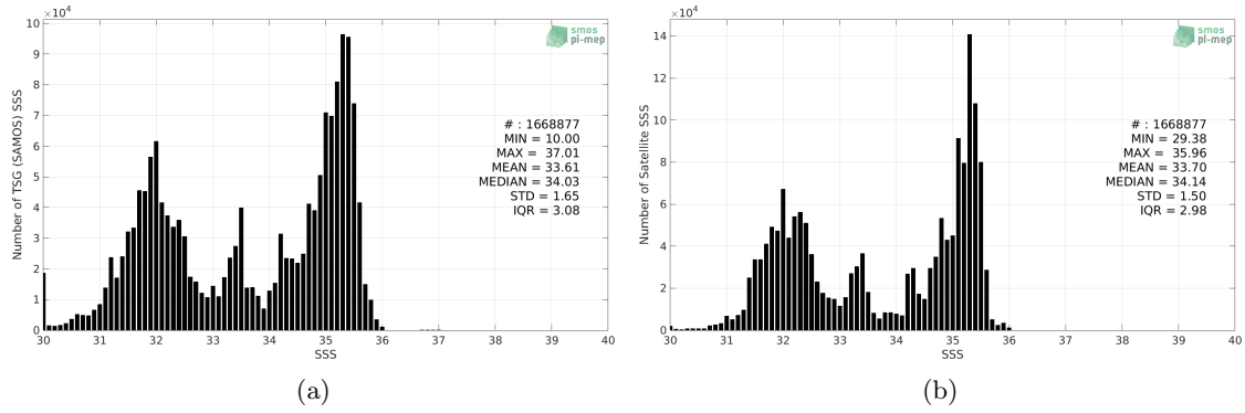
Figure 2: Histograms of SSS from TSG (SAMOS) (a) and Aquarius SSS L4 OI v5 - Monthly (IPRC) (b) considering all match-up pairs per bins of 0.1 over the Pacific Ocean Pi-MEP region and for the full satellite product period.
