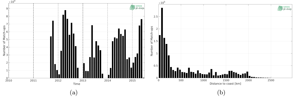
Figure 1: Number of match-ups between TSG (SAMOS) and Aquarius SSS L4 OI v5 - Monthly (IPRC) SSS as a function of time (a) and as function of the distance to coast (b) over the Pacific Ocean Pi-MEP region and for the full satellite product period.
