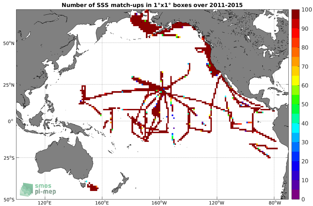
Figure 4: Number of SSS match-ups between TSG (SAMOS) SSS and the Aquarius SSS L4 OI v5 - Monthly (IPRC) SSS product for the Pacific Ocean Pi-MEP region over 1^\circ \times 1^\circ boxes and for the full satellite product period.
