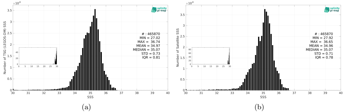
Figure 3: Histograms of SSS from TSG (LEGOS-DM) (a) and Aquarius SSS L4 OI v5 - Monthly (IPRC) (b) considering all match-up pairs per bins of 0.1 over the Pacific Ocean Pi-MEP region and for the full satellite product period.
