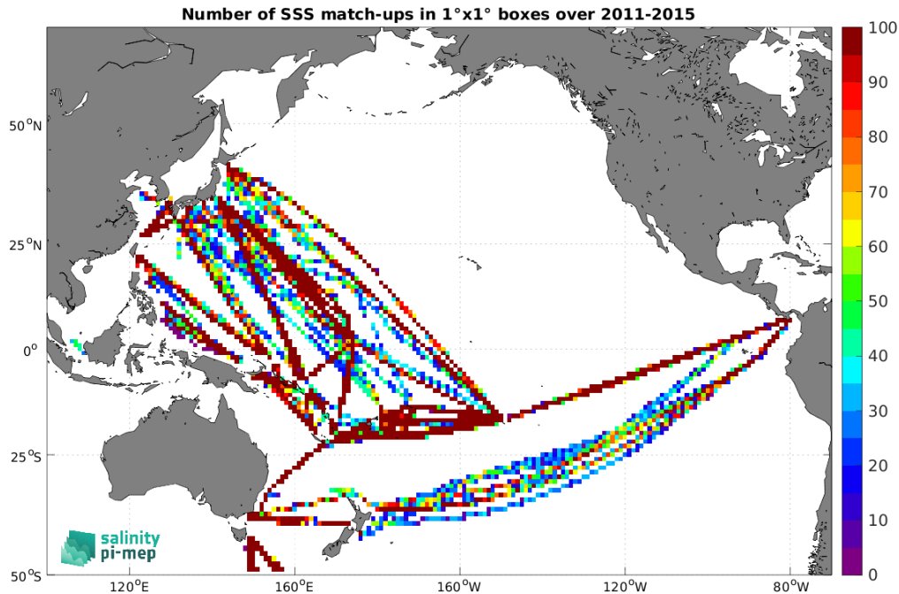
Figure 5: Number of SSS match-ups between TSG (LEGOS-DM) SSS and the Aquarius SSS L4 OI v5 - Monthly (IPRC) SSS product for the Pacific Ocean Pi-MEP region over 1^\circ \times 1^\circ boxes and for the full satellite product period.
