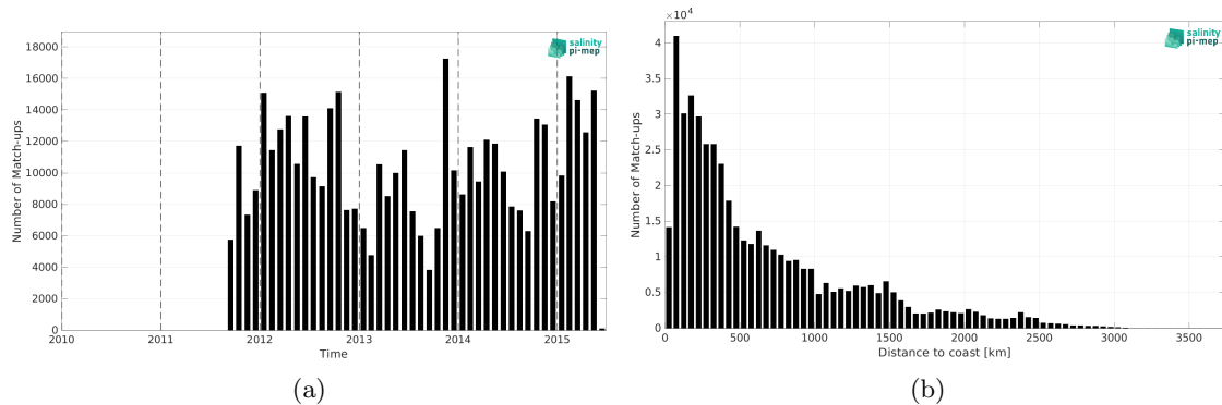
Figure 2: Number of match-ups between TSG (LEGOS-DM) and Aquarius SSS L4 OI v5 - Monthly (IPRC) SSS as a function of time (a) and as function of the distance to coast (b) over the Pacific Ocean Pi-MEP region and for the full satellite product period.
