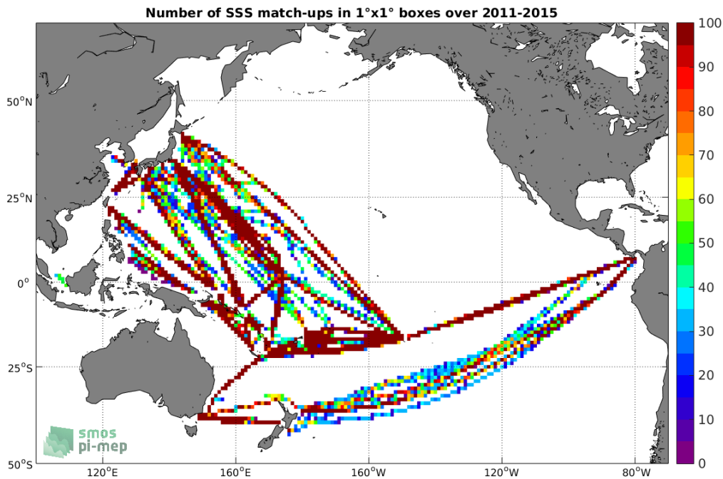
Figure 4: Number of SSS match-ups between TSG-LEGOS-DM SSS and the Aquarius-L4-IPRC-V5-MONTHLY SSS product for the Pacific Ocean Pi-MEP region over 1^\circ \times 1^\circ boxes and for the full satellite product period.
