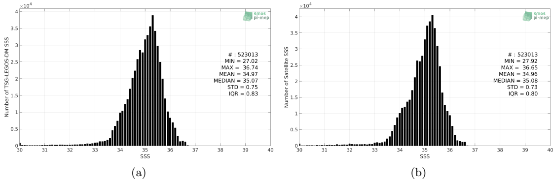
Figure 2: Histograms of SSS from TSG-LEGOS-DM (a) and Aquarius-L4-IPRC-V5-MONTHLY (b) considering all match-up pairs per bins of 0.1 over the Pacific Ocean Pi-MEP region and for the full satellite product period.
