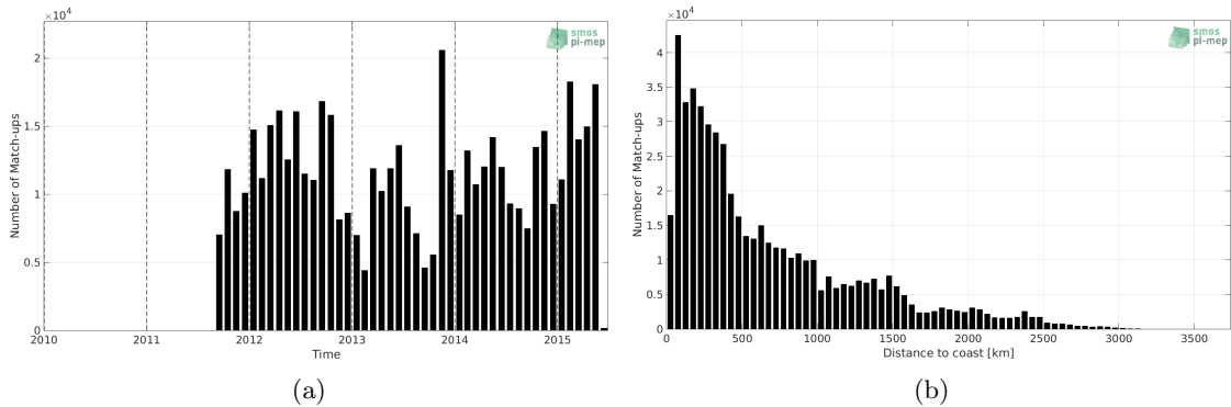
Figure 1: Number of match-ups between TSG-LEGOS-DM and Aquarius-L4-IPRC-V5-MONTHLY SSS as a function of time (a) and as function of the distance to coast (b) over the Pacific Ocean Pi-MEP region and for the full satellite product period.
