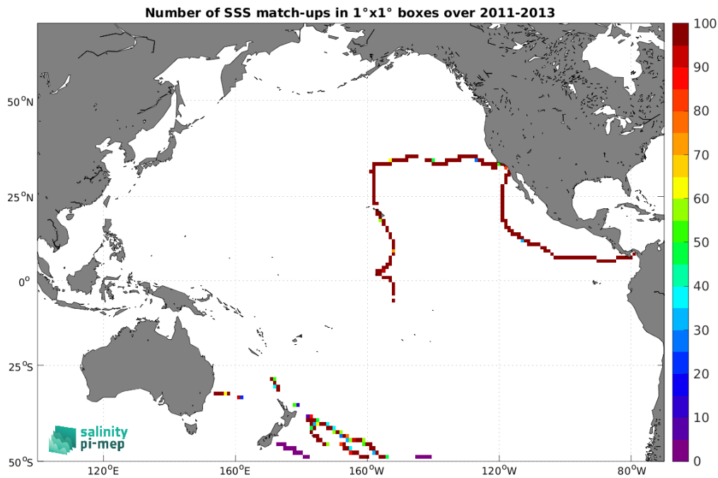
Figure 5: Number of SSS match-ups between TSG (GOSUD-Sailing-ship) SSS and the Aquarius SSS L4 OI v5 - Monthly (IPRC) SSS product for the Pacific Ocean Pi-MEP region over 1^\circ \times 1^\circ boxes and for the full satellite product period.
