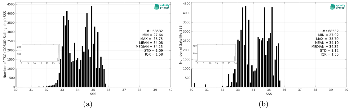
Figure 3: Histograms of SSS from TSG (GOSUD-Sailing-ship) (a) and Aquarius SSS L4 OI v5 - Monthly (IPRC) (b) considering all match-up pairs per bins of 0.1 over the Pacific Ocean Pi-MEP region and for the full satellite product period.
