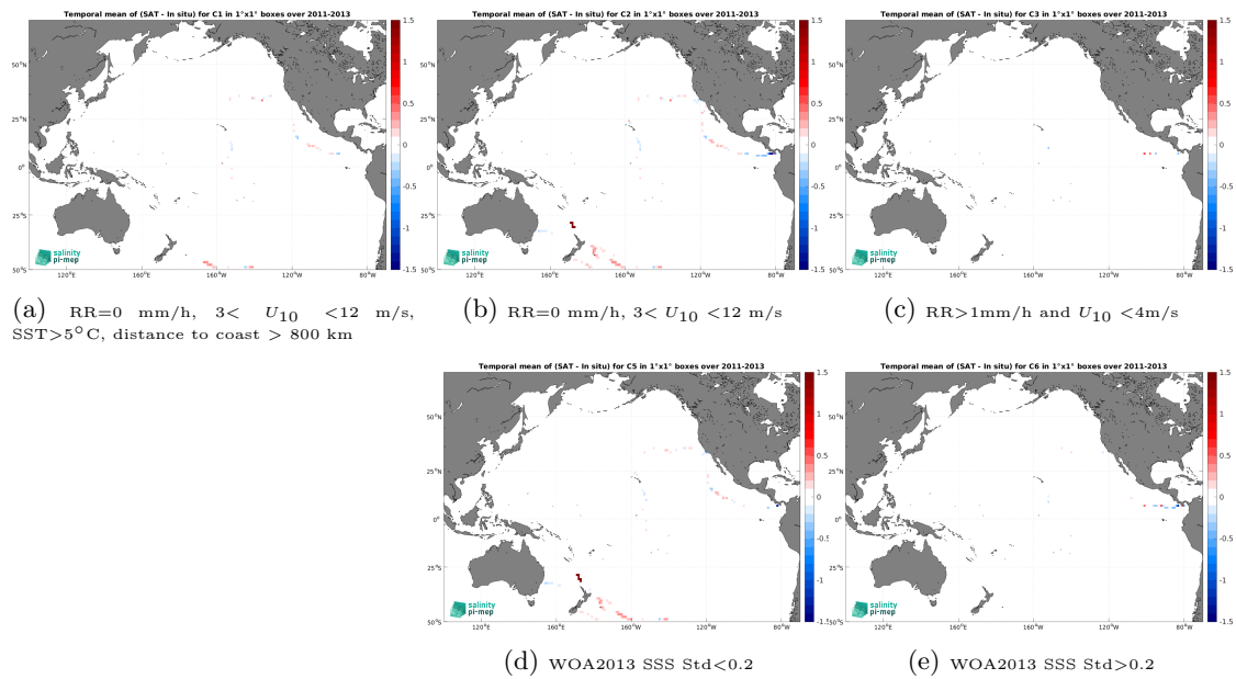
Figure 14: Temporal mean gridded over spatial boxes of size 1^\circ \times 1^\circ of \Delta\text{SSS} (Aquarius SSS L4 OI v5 - Monthly (IPRC) - TSG (GOSUD-Sailing-ship)) for 5 different subdatasets corresponding to: RR=0 mm/h, 3 < U_{10} < 12 m/s, SST > 5^\circ\text{C} , distance to coast > 800 km (a), RR=0 mm/h, 3 < U_{10} < 12 m/s (b), RR > 1 mm/h and U_{10} < 4 m/s (c), WOA2013 SSS Std < 0.2 (d), WOA2013 SSS Std > 0.2 (e).
