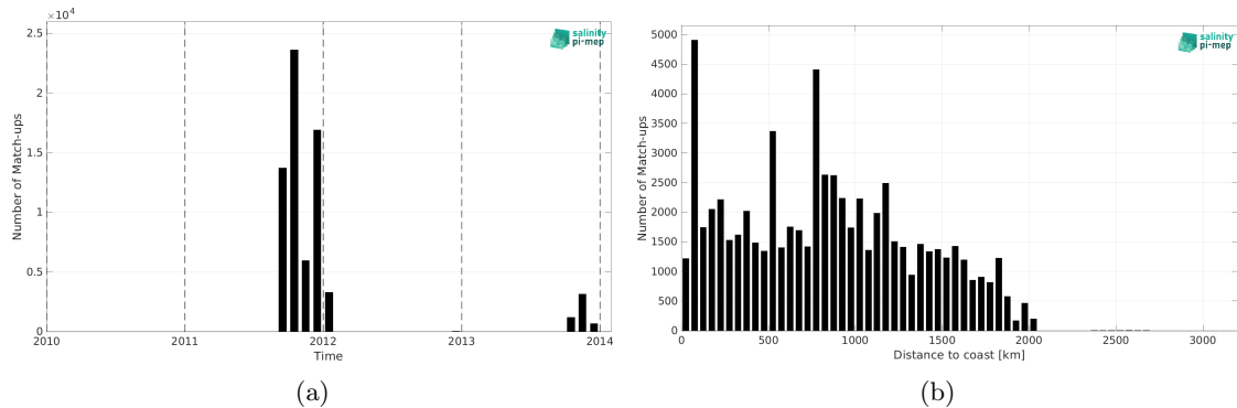
Figure 2: Number of match-ups between TSG (GOSUD-Sailing-ship) and Aquarius SSS L4 OI v5 - Monthly (IPRC) SSS as a function of time (a) and as function of the distance to coast (b) over the Pacific Ocean Pi-MEP region and for the full satellite product period.
