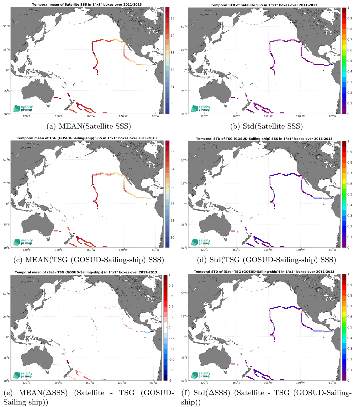
Figure 7: Temporal mean (left) and Std (right) of SSS from Aquarius SSS L4 OI v5 - Monthly (IPRC) (top), TSG (GOSUD-Sailing-ship) (middle), and of \Delta SSS (Satellite - TSG (GOSUD-Sailing-ship)). Only match-up pairs are used to generate these maps.
