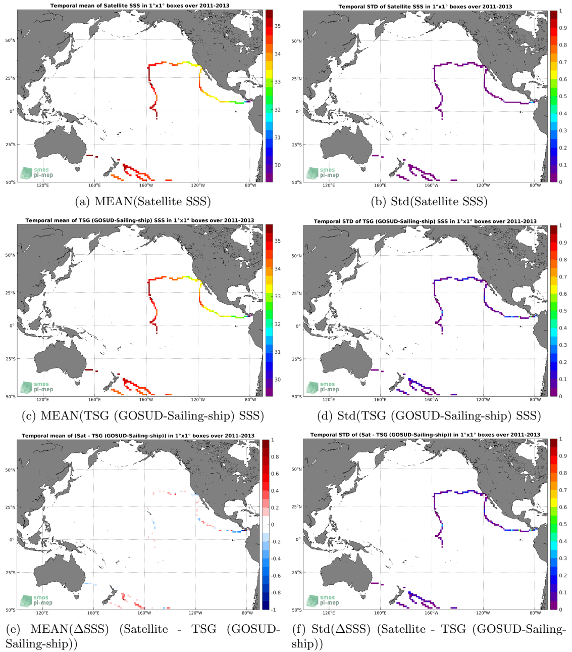
Figure 6: Temporal mean (left) and Std (right) of SSS from Aquarius SSS L4 OI v5 - Monthly (IPRC) (top), TSG (GOSUD-Sailing-ship) (middle), and of \Delta SSS (Satellite - TSG (GOSUD-Sailing-ship)). Only match-up pairs are used to generate these maps.
