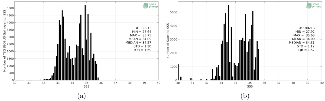
Figure 2: Histograms of SSS from TSG (GOSUD-Sailing-ship) (a) and Aquarius SSS L4 OI v5 - Monthly (IPRC) (b) considering all match-up pairs per bins of 0.1 over the Pacific Ocean Pi-MEP region and for the full satellite product period.
