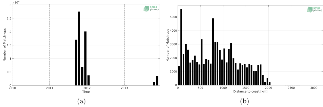
Figure 1: Number of match-ups between TSG (GOSUD-Sailing-ship) and Aquarius SSS L4 OI v5 - Monthly (IPRC) SSS as a function of time (a) and as function of the distance to coast (b) over the Pacific Ocean Pi-MEP region and for the full satellite product period.
