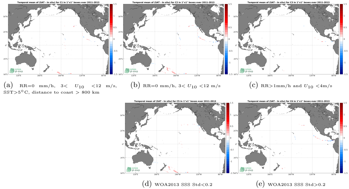
Figure 12: Temporal mean gridded over spatial boxes of size 1^\circ \times 1^\circ of \Delta SSS (Aquarius SSS L4 OI v5 - Monthly (IPRC) - TSG (GOSUD-Sailing-ship)) for 5 different subdatasets corresponding to: RR=0 mm/h, 3 < U_{10} < 12 m/s, SST >5^\circ C, distance to coast > 800 km (a), RR=0 mm/h, 3 < U_{10} < 12 m/s (b), RR >1 mm/h and U_{10} < 4 m/s (c), WOA2013 SSS Std <0.2 (d), WOA2013 SSS Std >0.2 (e).
