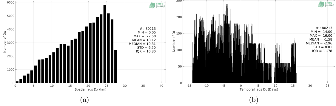
Figure 5: Histograms of the spatial (a) and temporal (b) lags between the time of the TSG (GOSUD-Sailing-ship) measurements and the date of the corresponding Aquarius SSS L4 OI v5 - Monthly (IPRC) SSS product.
