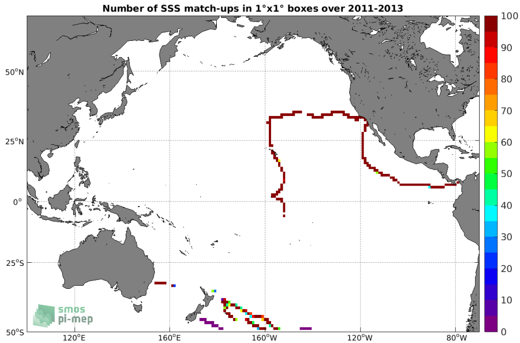
Figure 4: Number of SSS match-ups between TSG (GOSUD-Sailing-ship) SSS and the Aquarius SSS L4 OI v5 - Monthly (IPRC) SSS product for the Pacific Ocean Pi-MEP region over 1^\circ \times 1^\circ boxes and for the full satellite product period.
