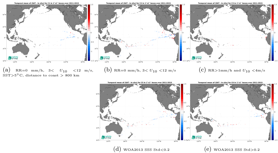
Figure 14: Temporal mean gridded over spatial boxes of size 1^\circ \times 1^\circ of \Delta SSS (Aquarius SSS L4 OI v5 - Monthly (IPRC) - TSG (GOSUD-Research-vessel)) for 5 different subdatasets corresponding to: RR=0 mm/h, 3 < U_{10} < 12 m/s, SST > 5^\circ\text{C} , distance to coast > 800 km (a), RR=0 mm/h, 3 < U_{10} < 12 m/s (b), RR > 1 mm/h and U_{10} < 4 m/s (c), WOA2013 SSS Std < 0.2 (d), WOA2013 SSS Std > 0.2 (e).
