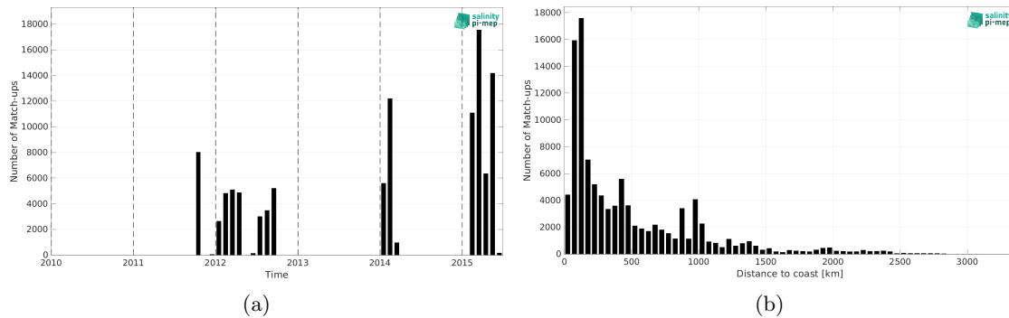
Figure 2: Number of match-ups between TSG (GOSUD-Research-vessel) and Aquarius SSS L4 OI v5 - Monthly (IPRC) SSS as a function of time (a) and as function of the distance to coast (b) over the Pacific Ocean Pi-MEP region and for the full satellite product period.
