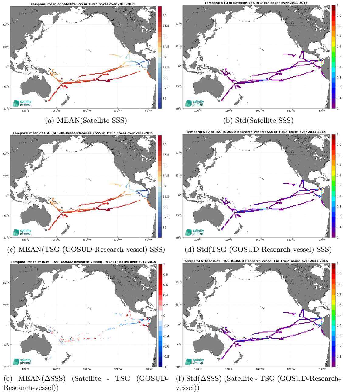
Figure 7: Temporal mean (left) and Std (right) of SSS from Aquarius SSS L4 OI v5 - Monthly (IPRC) (top), TSG (GOSUD-Research-vessel) (middle), and of \Delta SSS (Satellite - TSG (GOSUD-Research-vessel)). Only match-up pairs are used to generate these maps.
