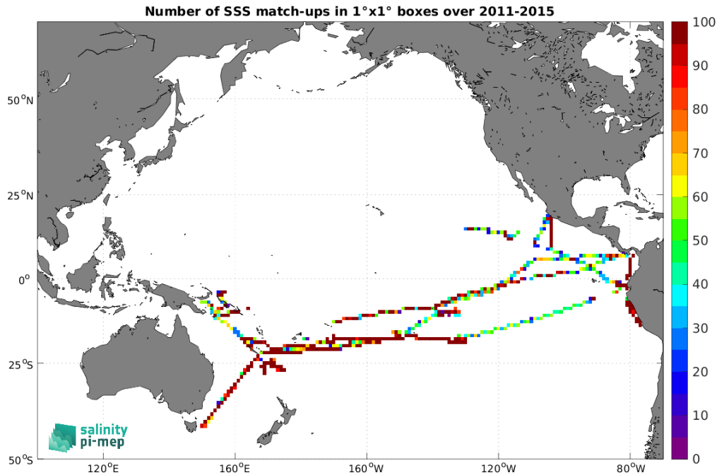
Figure 5: Number of SSS match-ups between TSG (GOSUD-Research-vessel) SSS and the Aquarius SSS L4 OI v5 - Monthly (IPRC) SSS product for the Pacific Ocean Pi-MEP region over 1^\circ \times 1^\circ boxes and for the full satellite product period.
