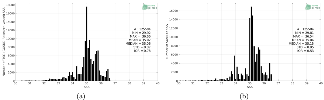
Figure 2: Histograms of SSS from TSG (GOSUD-Research-vessel) (a) and Aquarius SSS L4 OI v5 - Monthly (IPRC) (b) considering all match-up pairs per bins of 0.1 over the Pacific Ocean Pi-MEP region and for the full satellite product period.
