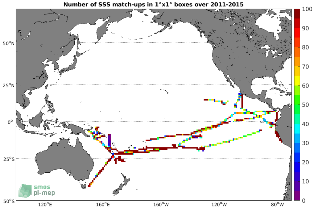
Figure 4: Number of SSS match-ups between TSG (GOSUD-Research-vessel) SSS and the Aquarius SSS L4 OI v5 - Monthly (IPRC) SSS product for the Pacific Ocean Pi-MEP region over 1°x1° boxes and for the full satellite product period.
