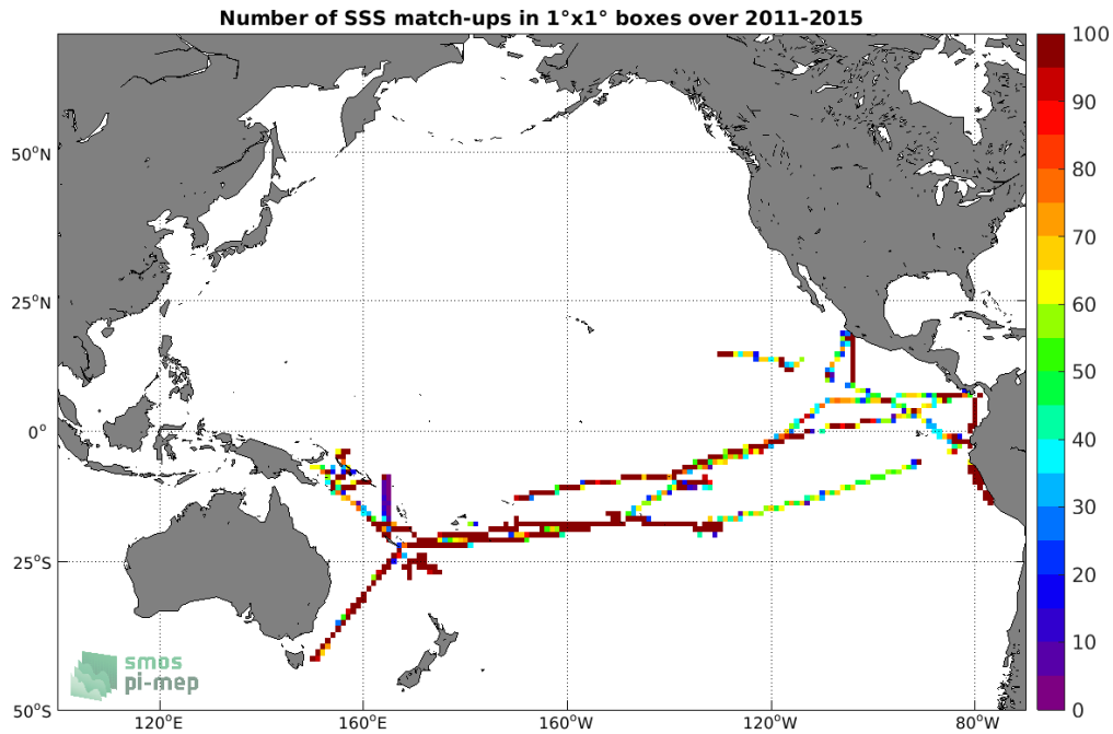
Figure 4: Number of SSS match-ups between TSG (GOSUD-Research-vessel) SSS and the Aquarius SSS L4 OI v5 - Monthly (IPRC) SSS product for the Pacific Ocean Pi-MEP region over 1^\circ \times 1^\circ boxes and for the full satellite product period.
