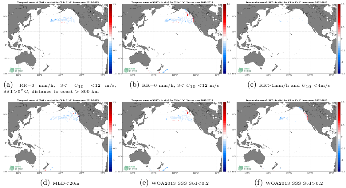
Figure 12: Temporal mean gridded over spatial boxes of size 1^\circ \times 1^\circ of \Delta SSS (Aquarius SSS L4 OI v5 - Monthly (IPRC) - Sea mammals) for 6 different subdatasets corresponding to: RR=0 mm/h, 3 < U_{10} < 12 m/s, SST > 5^\circ C , distance to coast > 800 km (a), RR=0 mm/h, 3 < U_{10} < 12 m/s (b), RR > 1 mm/h and U_{10} < 4 m/s (c), MLD < 20 m (d), WOA2013 SSS Std < 0.2 (e), WOA2013 SSS Std > 0.2 (f).
