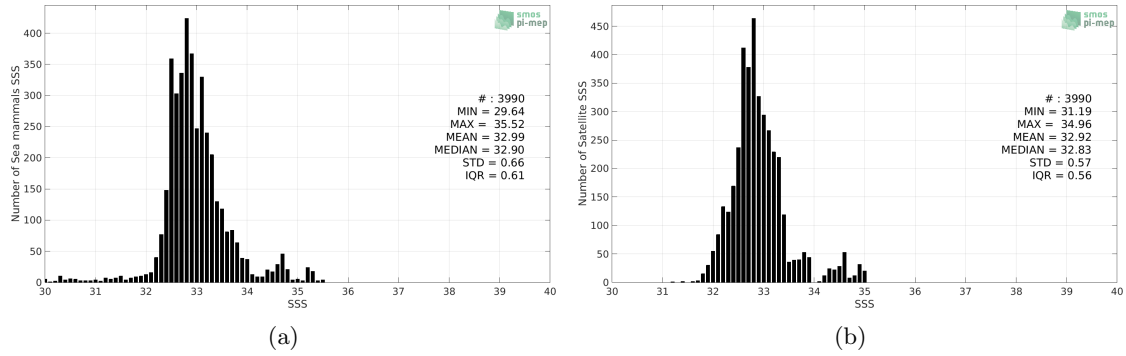
Figure 2: Histograms of SSS from Sea mammals (a) and Aquarius SSS L4 OI v5 - Monthly (IPRC) (b) considering all match-up pairs per bins of 0.1 over the Pacific Ocean Pi-MEP region and for the full satellite product period.
