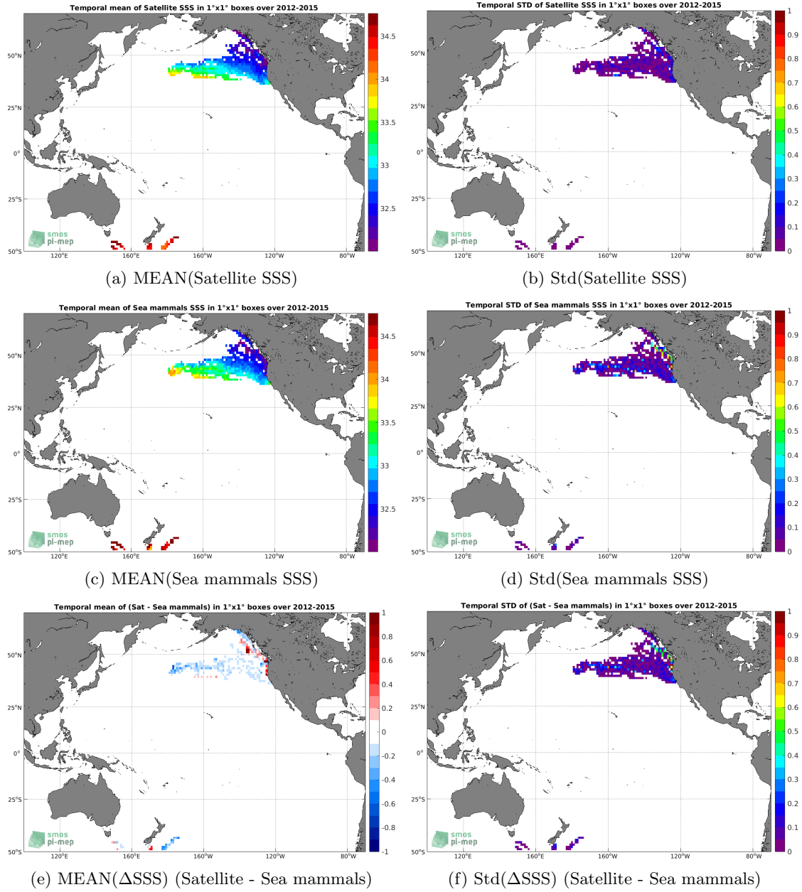
Figure 6: Temporal mean (left) and Std (right) of SSS from Aquarius SSS L4 OI v5 - Monthly (IPRC) (top), Sea mammals (middle), and of \Delta SSS (Satellite - Sea mammals). Only match-up pairs are used to generate these maps.
