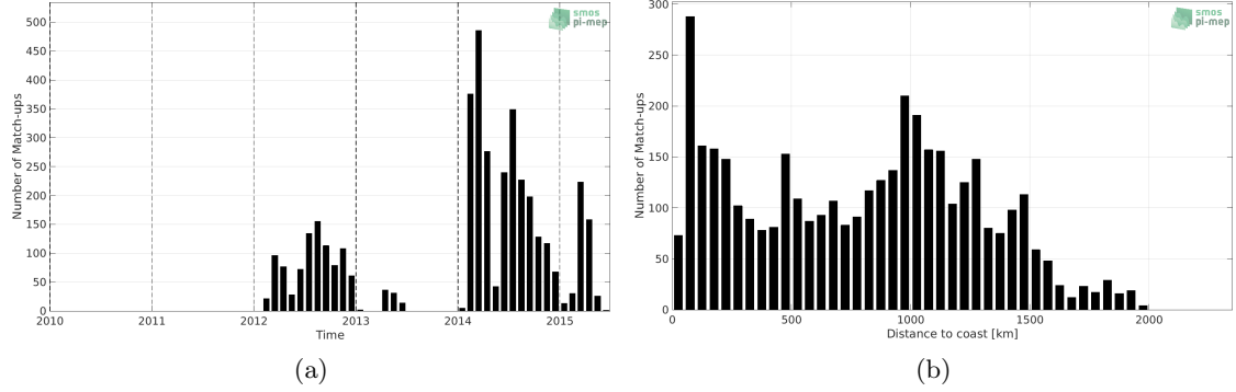
Figure 1: Number of match-ups between Sea mammals and Aquarius SSS L4 OI v5 - Monthly (IPRC) SSS as a function of time (a) and as function of the distance to coast (b) over the Pacific Ocean Pi-MEP region and for the full satellite product period.
