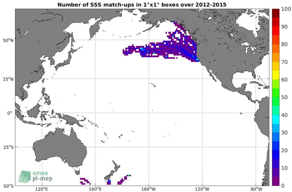
Figure 4: Number of SSS match-ups between Sea mammals SSS and the Aquarius SSS L4 OI v5 - Monthly (IPRC) SSS product for the Pacific Ocean Pi-MEP region over 1°x1° boxes and for the full satellite product period.
