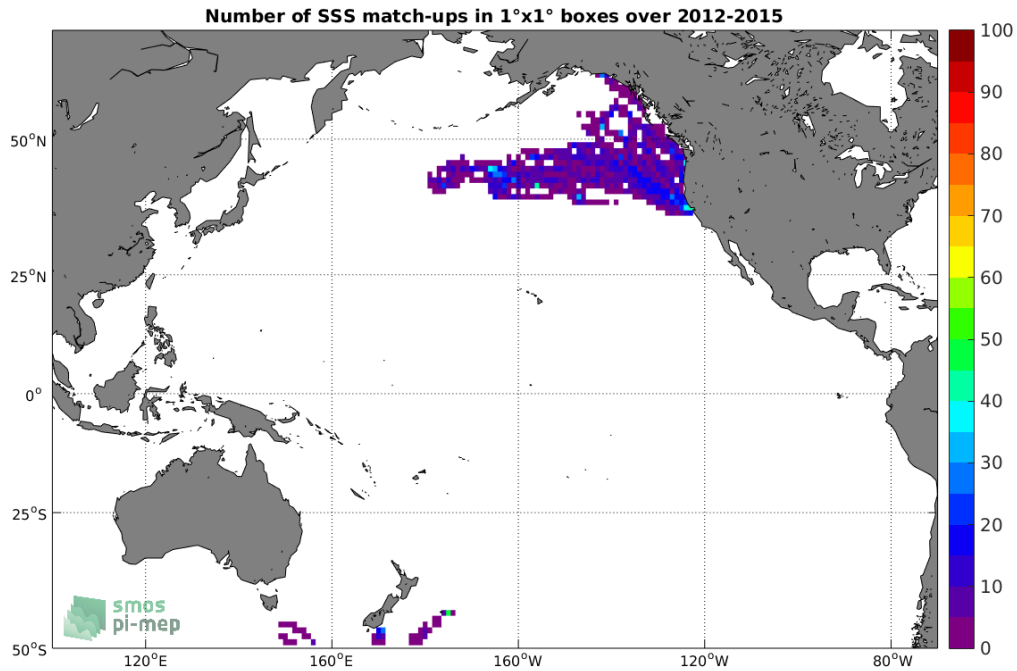
Figure 4: Number of SSS match-ups between Sea mammals SSS and the Aquarius-L4-IPRC-V5-MONTHLY SSS product for the Pacific Ocean Pi-MEP region over 1^\circ \times 1^\circ boxes and for the full satellite product period.
