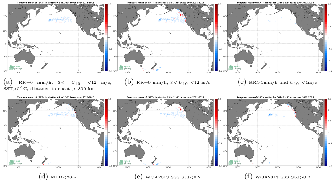
Figure 12: Temporal mean gridded over spatial boxes of size 1^\circ \times 1^\circ of \Delta SSS (Aquarius-L4-IPRC-V5-MONTHLY - Sea mammals) for 6 different subdatasets corresponding to: RR=0 mm/h, 3 < U_{10} < 12 m/s, SST > 5^\circ C , distance to coast > 800 km (a), RR=0 mm/h, 3 < U_{10} < 12 m/s (b), RR > 1 mm/h and U_{10} < 4 m/s (c), MLD < 20 m (d), WOA2013 SSS Std < 0.2 (e), WOA2013 SSS Std > 0.2 (f).
