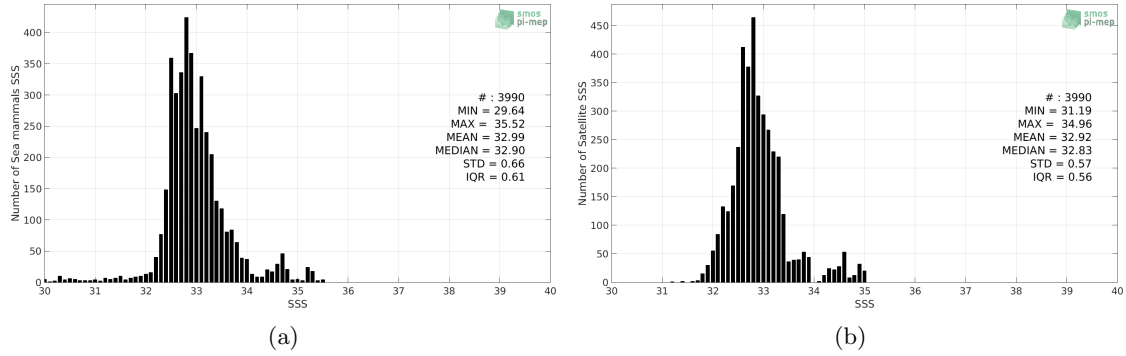
Figure 2: Histograms of SSS from Sea mammals (a) and Aquarius-L4-IPRC-V5-MONTHLY (b) considering all match-up pairs per bins of 0.1 over the Pacific Ocean Pi-MEP region and for the full satellite product period.
