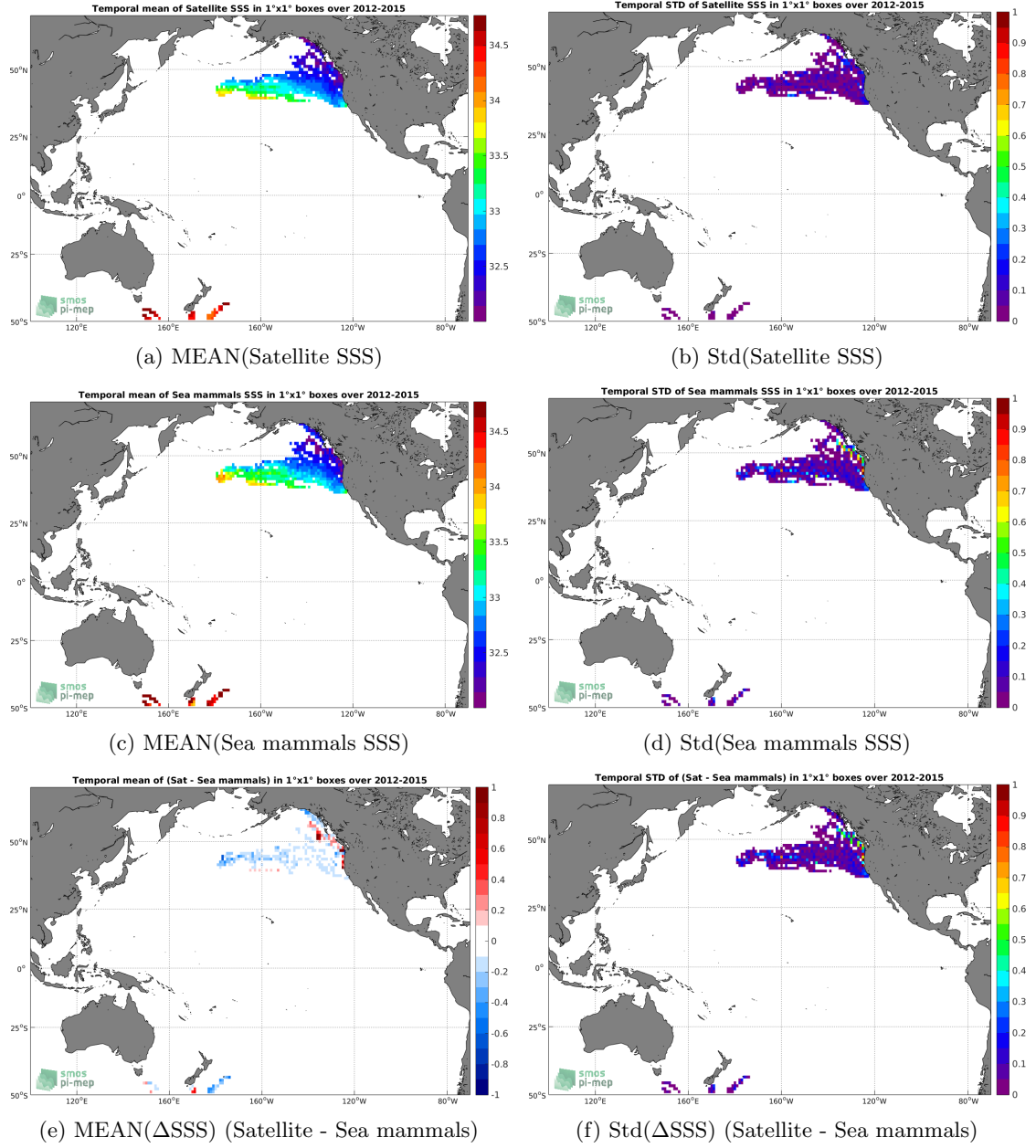
Figure 6: Temporal mean (left) and Std (right) of SSS from Aquarius-L4-IPRC-V5-MONTHLY (top), Sea mammals (middle), and of \Delta SSS (Satellite - Sea mammals). Only match-up pairs are used to generate these maps.
