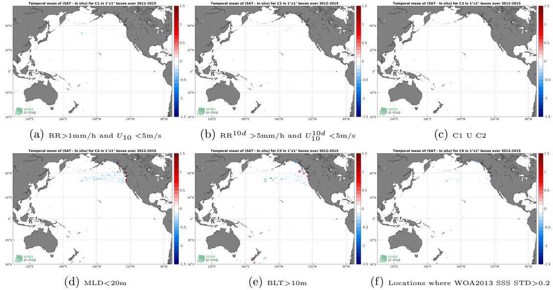
Figure 12: Temporal mean gridded over spatial boxes of size 1^\circ \times 1^\circ of \Delta\text{SSS} (Aquarius-L4-IPRC-V5-MONTHLY - Sea mammals) for 6 different subdatasets corresponding to: RR > 1\text{mm/h} and U_{10} < 5\text{m/s} (a), RR^{10d} > 5\text{mm/h} and U_{10}^{10d} < 5\text{m/s} (b), C1 U C2 (c), MLD < 20\text{m} (d), BLT > 10\text{m} (e), Locations where WOA2013 SSS STD > 0.2 (f).
