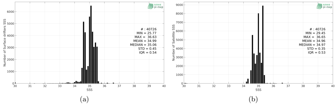
Figure 2: Histograms of SSS from Surface drifters (a) and Aquarius-L4-IPRC-V5-MONTHLY (b) considering all match-up pairs per bins of 0.1 over the Pacific Ocean Pi-MEP region and for the full satellite product period.
