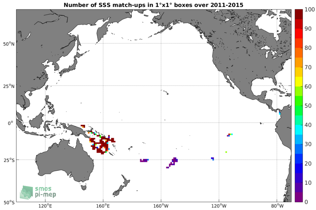
Figure 3: Number of SSS match-ups between Surface drifters SSS and the Aquarius-L4-IPRC-V5-MONTHLY SSS product for the Pacific Ocean Pi-MEP region over 1^\circ \times 1^\circ boxes and for the full satellite product period.
