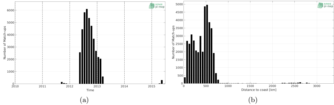
Figure 1: Number of match-ups between Surface drifters and Aquarius-L4-IPRC-V5-MONTHLY SSS as a function of time (a) and as function of the distance to coast (b) over the Pacific Ocean Pi-MEP region and for the full satellite product period.
