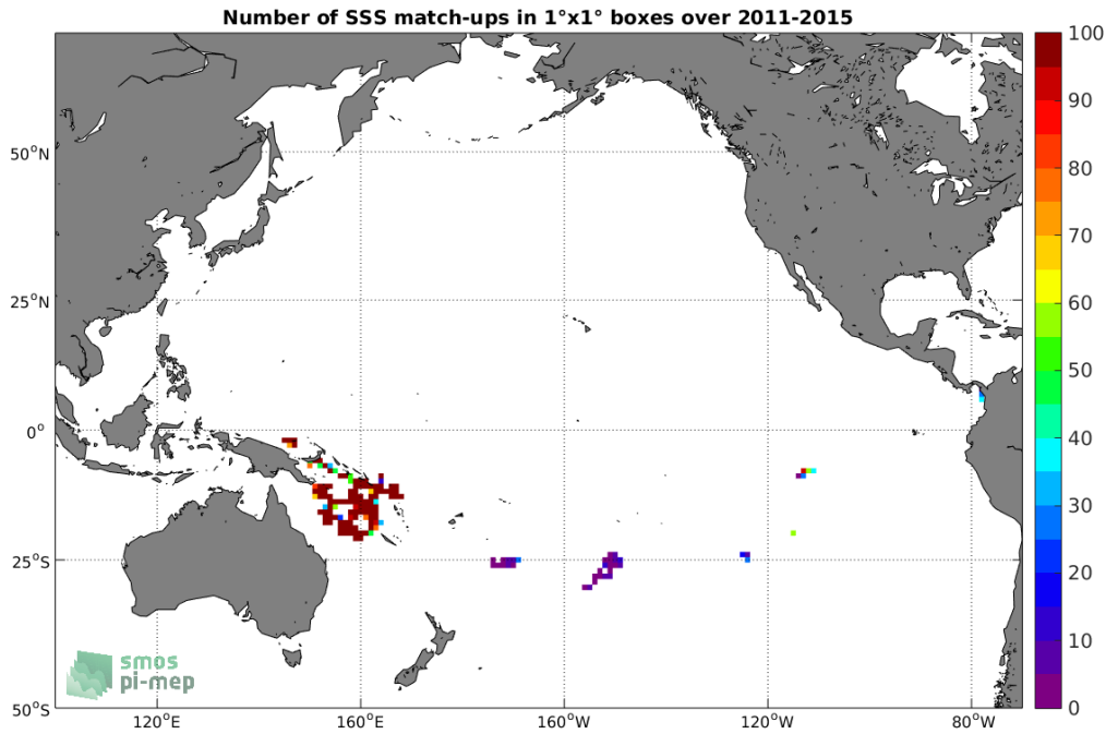
Figure 3: Number of SSS match-ups between Surface drifters SSS and the Aquarius-L4-IPRC-V5-MONTHLY SSS product for the Pacific Ocean Pi-MEP region over 1°x1° boxes and for the full satellite product period.
