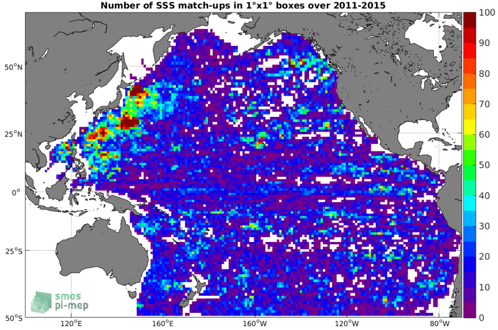
Figure 4: Number of SSS match-ups between Argo SSS and the Aquarius SSS L4 OI v5 - Monthly (IPRC) SSS product for the Pacific Ocean Pi-MEP region over 1^\circ \times 1^\circ boxes and for the full satellite product period.
