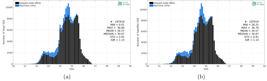
Figure 2: Histograms of SSS from Argo (a) and Aquarius SSS L4 OI v5 - Monthly (IPRC) (b) considering all match-up pairs per bins of 0.1 over the Pacific Ocean Pi-MEP region and for the full satellite product period.
