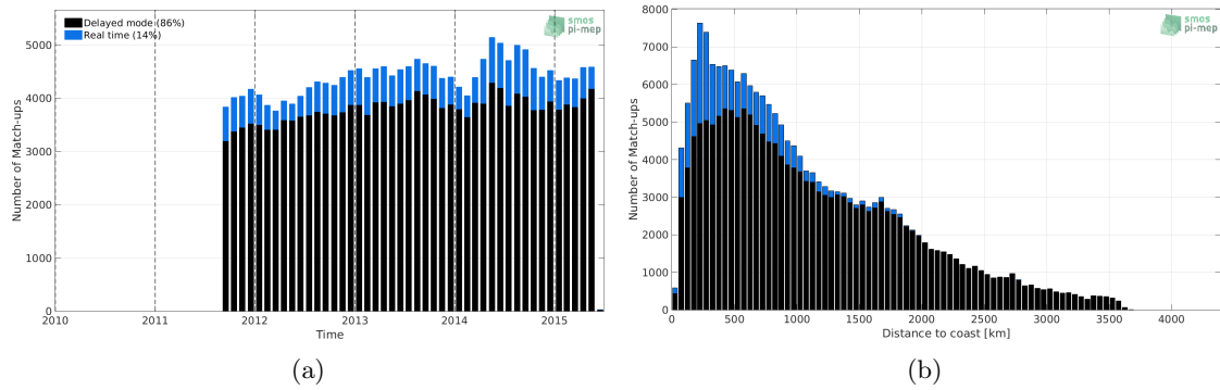
Figure 1: Number of match-ups between Argo and Aquarius SSS L4 OI v5 - Monthly (IPRC) SSS as a function of time (a) and as function of the distance to coast (b) over the Pacific Ocean Pi-MEP region and for the full satellite product period.
