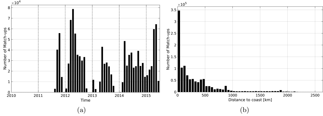
Figure 1: Number of match-ups between TSG-SAMOS and Aquarius-L4-IPRC-V4-WEEKLY SSS as a function of time (a) and as function of the distance to coast (b) over the Pacific Ocean Pi-MEP region and for the full satellite product period.
