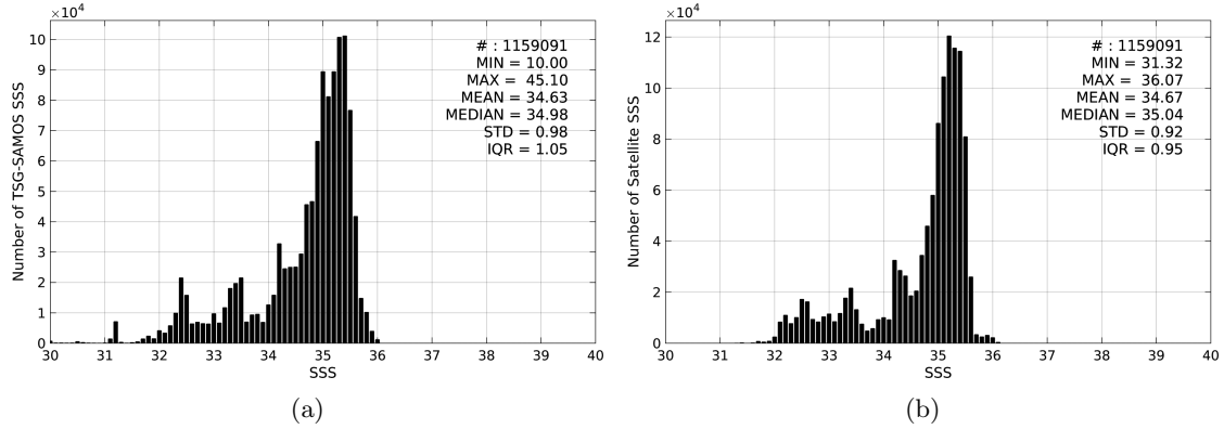
Figure 2: Histograms of SSS from TSG-SAMOS (a) and Aquarius-L4-IPRC-V4-WEEKLY (b) considering all match-up pairs per bins of 0.1 over the Pacific Ocean Pi-MEP region and for the full satellite product period.
