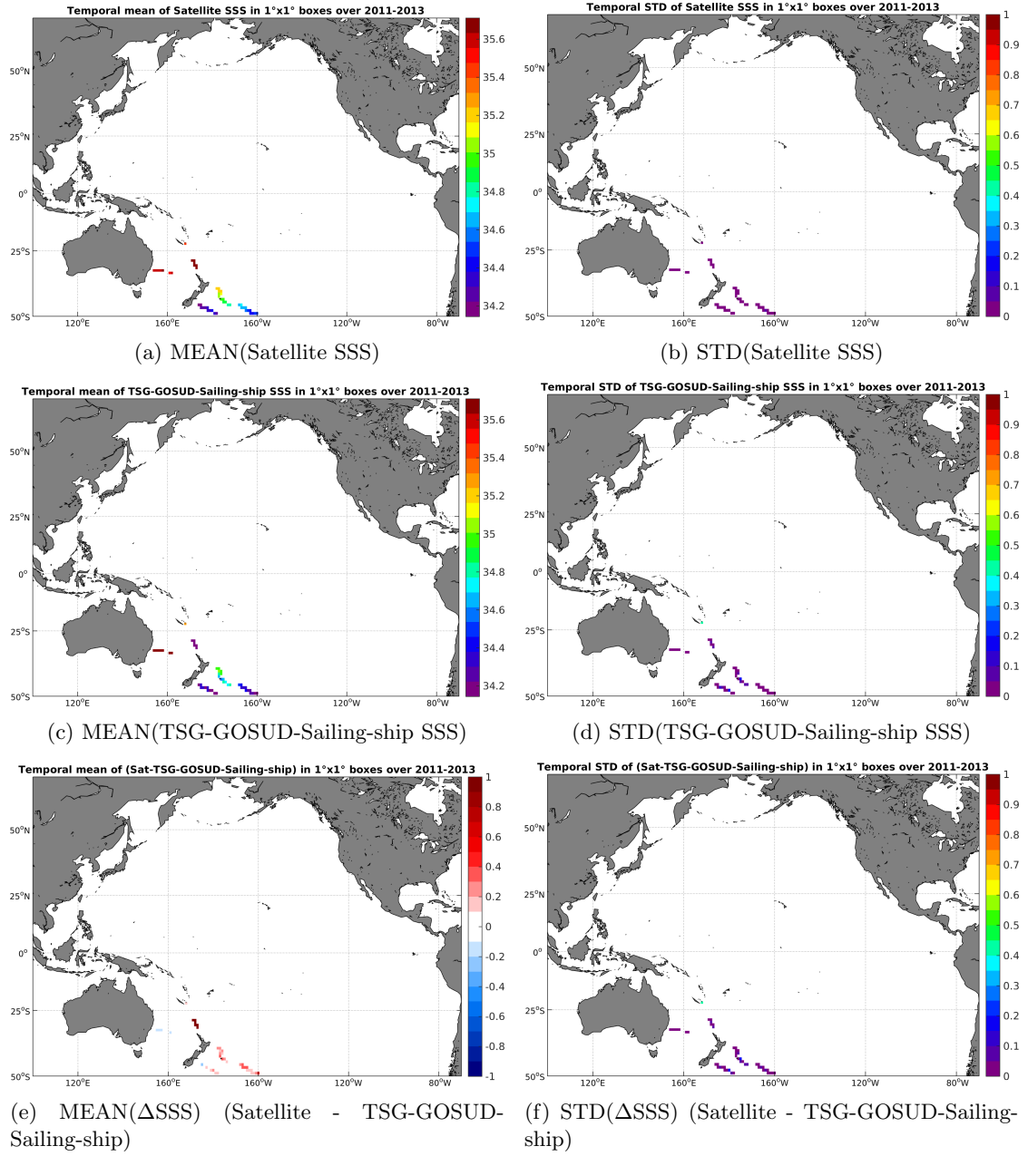
Figure 6: Temporal mean (left) and STD (right) of SSS from Aquarius-L4-IPRC-V4-WEEKLY (top), TSG-GOSUD-Sailing-ship (middle), and of \Delta SSS (Satellite - TSG-GOSUD-Sailing-ship). Only match-up pairs are used to generate these maps.
