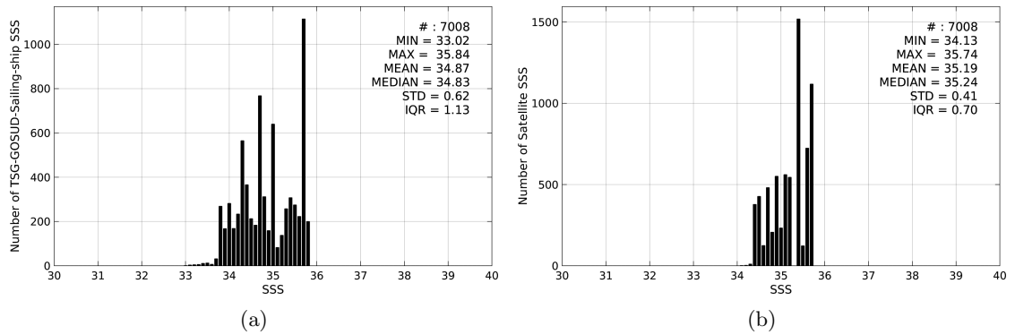
Figure 2: Histograms of SSS from TSG-GOSUD-Sailing-ship (a) and Aquarius-L4-IPRC-V4-WEEKLY (b) considering all match-up pairs per bins of 0.1 over the Pacific Ocean Pi-MEP region and for the full satellite product period.
