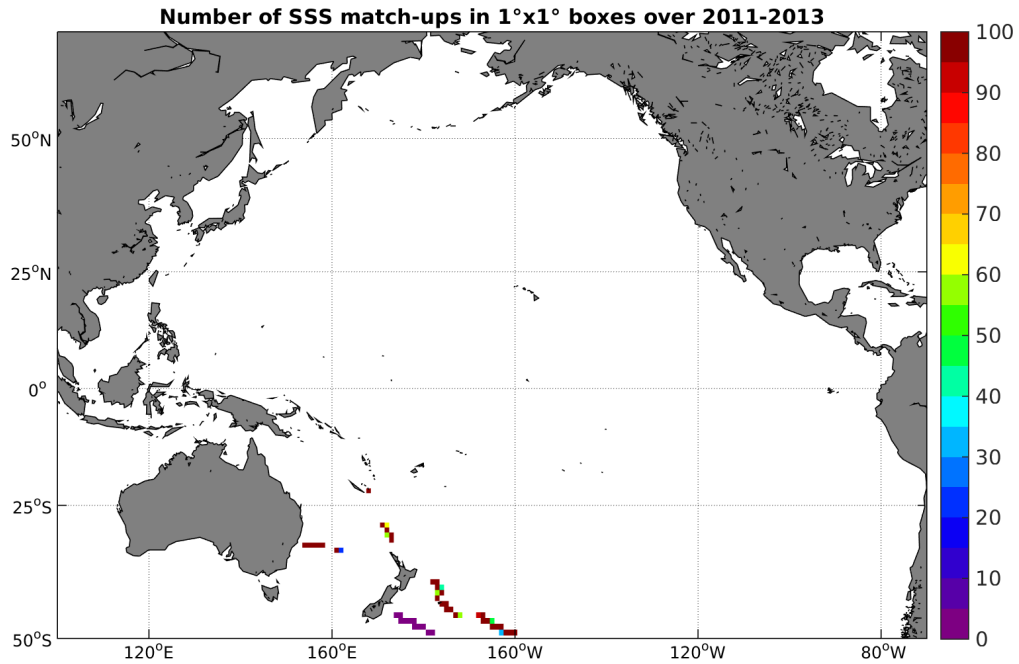
Figure 4: Number of SSS match-ups between TSG-GOSUD-Sailing-ship SSS and the Aquarius-L4-IPRC-V4-WEEKLY SSS product for the Pacific Ocean Pi-MEP region over 1^\circ \times 1^\circ boxes and for the full satellite product period.
