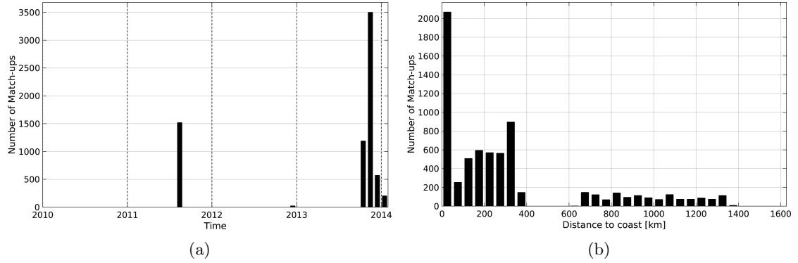
Figure 1: Number of match-ups between TSG-GOSUD-Sailing-ship and Aquarius-L4-IPRC-V4-WEEKLY SSS as a function of time (a) and as function of the distance to coast (b) over the Pacific Ocean Pi-MEP region and for the full satellite product period.
