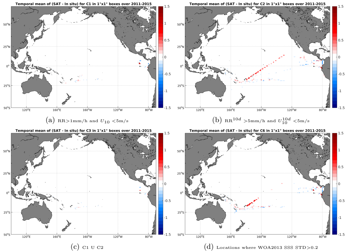
Figure 12: Temporal mean gridded over spatial boxes of size 1^\circ \times 1^\circ of \Delta SSS (Aquarius-L4-IPRC-V4-WEEKLY - TSG-GOSUD-Research-vessel) for 4 different subdatasets corresponding to: RR > 1\text{mm/h} and U_{10} < 5\text{m/s} (a), RR^{10d} > 5\text{mm/h} and U_{10}^{10d} < 5\text{m/s} (b), C1 U C2 (c), Locations where WOA2013 SSS STD > 0.2 (d).
