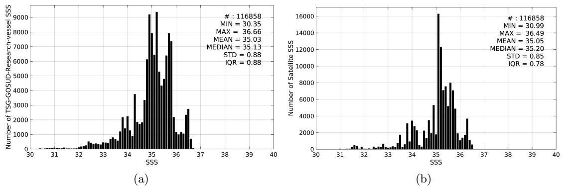
Figure 2: Histograms of SSS from TSG-GOSUD-Research-vessel (a) and Aquarius-L4-IPRC-V4-WEEKLY (b) considering all match-up pairs per bins of 0.1 over the Pacific Ocean Pi-MEP region and for the full satellite product period.
