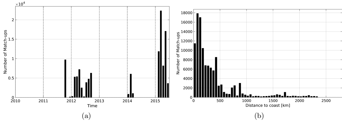
Figure 1: Number of match-ups between TSG-GOSUD-Research-vessel and Aquarius-L4-IPRC-V4-WEEKLY SSS as a function of time (a) and as function of the distance to coast (b) over the Pacific Ocean Pi-MEP region and for the full satellite product period.
