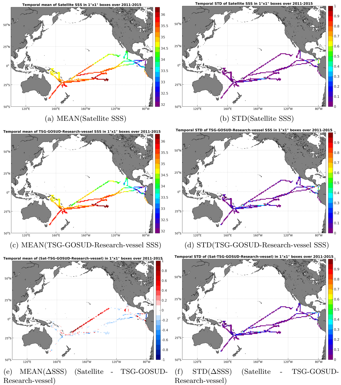
Figure 6: Temporal mean (left) and STD (right) of SSS from Aquarius-L4-IPRC-V4-WEEKLY (top), TSG-GOSUD-Research-vessel (middle), and of \Delta SSS (Satellite - TSG-GOSUD-Research-vessel). Only match-up pairs are used to generate these maps.
