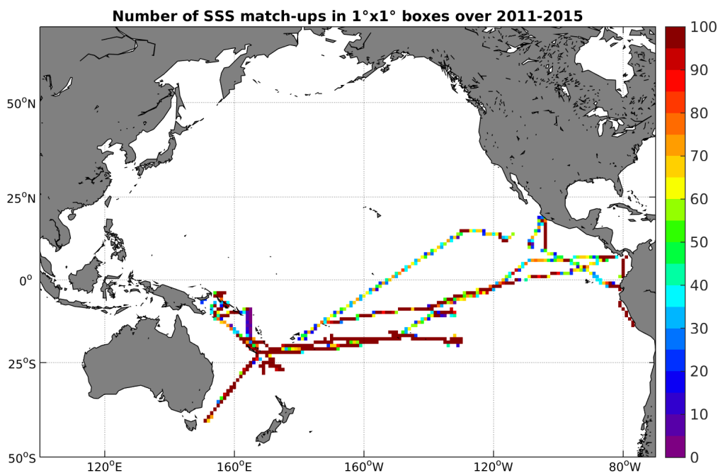
Figure 4: Number of SSS match-ups between TSG-GOSUD-Research-vessel SSS and the Aquarius-L4-IPRC-V4-WEEKLY SSS product for the Pacific Ocean Pi-MEP region over 1^\circ \times 1^\circ boxes and for the full satellite product period.
