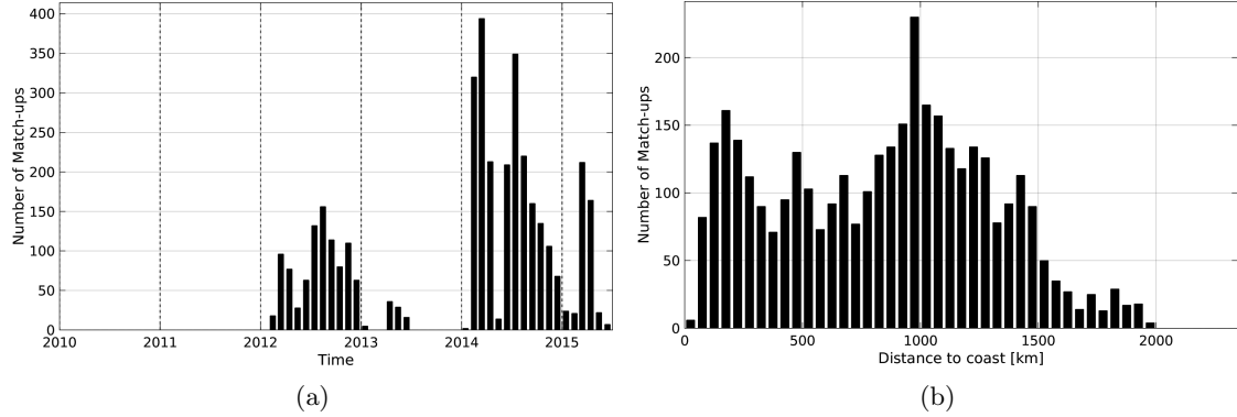
Figure 1: Number of match-ups between Sea mammals and Aquarius-L4-IPRC-V4-WEEKLY SSS as a function of time (a) and as function of the distance to coast (b) over the Pacific Ocean Pi-MEP region and for the full satellite product period.
