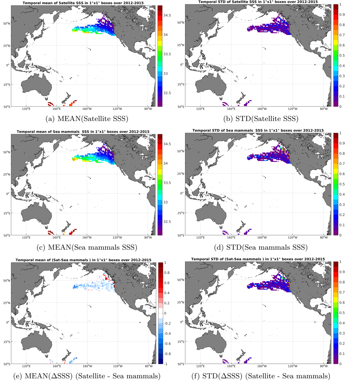
Figure 6: Temporal mean (left) and STD (right) of SSS from Aquarius-L4-IPRC-V4-WEEKLY (top), Sea mammals (middle), and of \Delta SSS (Satellite - Sea mammals). Only match-up pairs are used to generate these maps.
