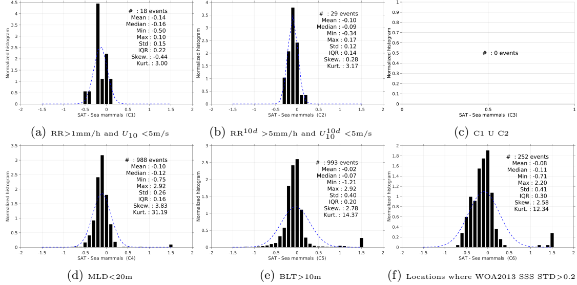
Figure 13: Normalized histogram of \Delta SSS (Aquarius-L4-IPRC-V4-WEEKLY - Sea mammals) for 6 different subdatasets corresponding to: RR > 1\text{mm/h} and U_{10} < 5\text{m/s} (a), RR^{10d} > 5\text{mm/h} and U_{10}^{10d} < 5\text{m/s} (b), C1 \cup C2 (c), MLD < 20\text{m} (d), BLT > 10\text{m} (e), Locations where WOA2013 SSS STD > 0.2 (f).
