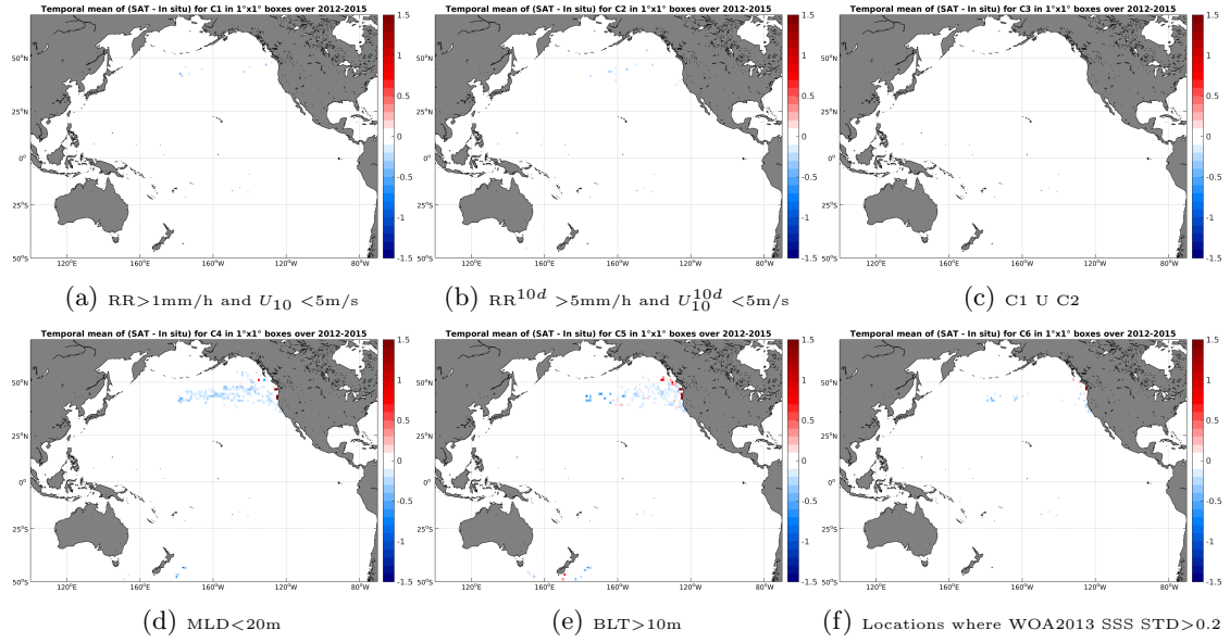
Figure 12: Temporal mean gridded over spatial boxes of size 1^\circ \times 1^\circ of \Delta SSS (Aquarius-L4-IPRC-V4-WEEKLY - Sea mammals) for 6 different subdatasets corresponding to: RR > 1\text{mm/h} and U_{10} < 5\text{m/s} (a), RR^{10d} > 5\text{mm/h} and U_{10}^{10d} < 5\text{m/s} (b), C1 U C2 (c), MLD < 20\text{m} (d), BLT > 10\text{m} (e), Locations where WOA2013 SSS STD > 0.2 (f).
