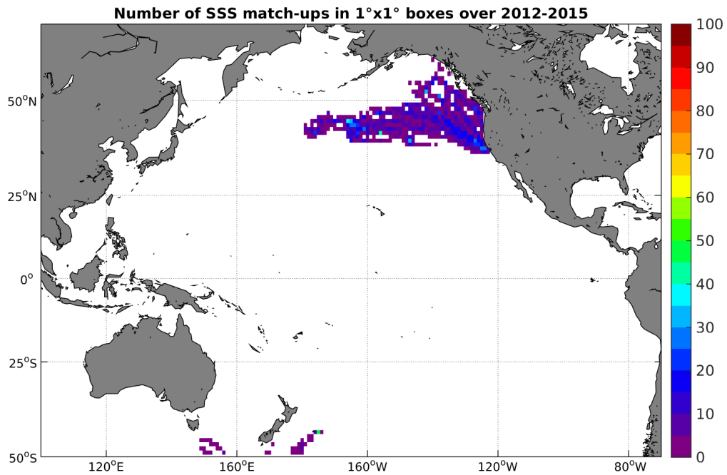
Figure 4: Number of SSS match-ups between Sea mammals SSS and the Aquarius-L4-IPRC-V4-WEEKLY SSS product for the Pacific Ocean Pi-MEP region over 1^\circ \times 1^\circ boxes and for the full satellite product period.
