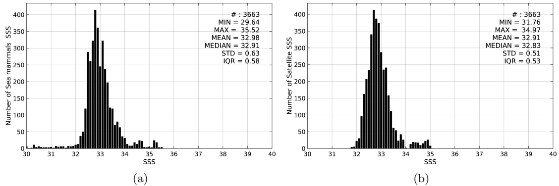
Figure 2: Histograms of SSS from Sea mammals (a) and Aquarius-L4-IPRC-V4-WEEKLY (b) considering all match-up pairs per bins of 0.1 over the Pacific Ocean Pi-MEP region and for the full satellite product period.
