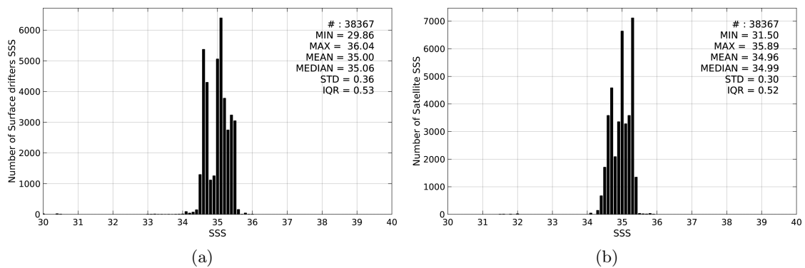
Figure 2: Histograms of SSS from Surface drifters (a) and Aquarius-L4-IPRC-V4-WEEKLY (b) considering all match-up pairs per bins of 0.1 over the Pacific Ocean Pi-MEP region and for the full satellite product period.
