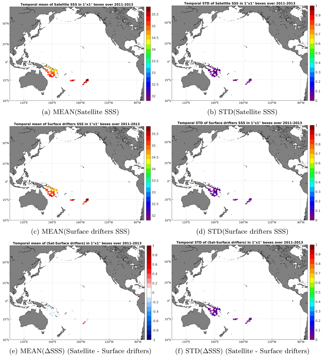
Figure 5: Temporal mean (left) and STD (right) of SSS from Aquarius-L4-IPRC-V4-WEEKLY (top), Surface drifters (middle), and of \Delta SSS (Satellite - Surface drifters). Only match-up pairs are used to generate these maps.
