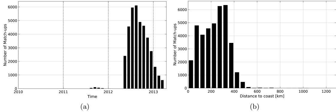
Figure 1: Number of match-ups between Surface drifters and Aquarius-L4-IPRC-V4-WEEKLY SSS as a function of time (a) and as function of the distance to coast (b) over the Pacific Ocean Pi-MEP region and for the full satellite product period.
