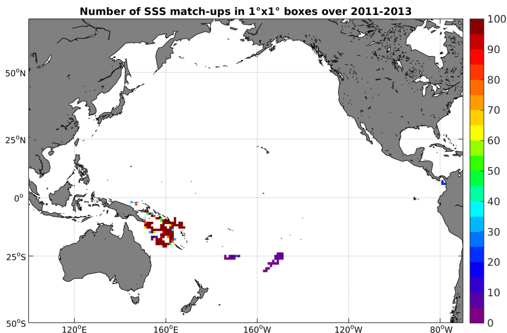
Figure 3: Number of SSS match-ups between Surface drifters SSS and the Aquarius-L4-IPRC-V4-WEEKLY SSS product for the Pacific Ocean Pi-MEP region over 1^\circ \times 1^\circ boxes and for the full satellite product period.
