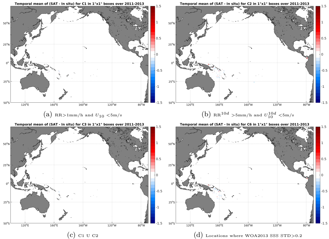
Figure 11: Temporal mean gridded over spatial boxes of size 1^\circ \times 1^\circ of \Delta SSS (Aquarius-L4-IPRC-V4-WEEKLY - Surface drifters) for 4 different subdatasets corresponding to: RR > 1\text{mm/h} and U_{10} < 5\text{m/s} (a), RR^{10d} > 5\text{mm/h} and U_{10}^{10d} < 5\text{m/s} (b), C1 U C2 (c), Locations where WOA2013 SSS STD > 0.2 (d).
