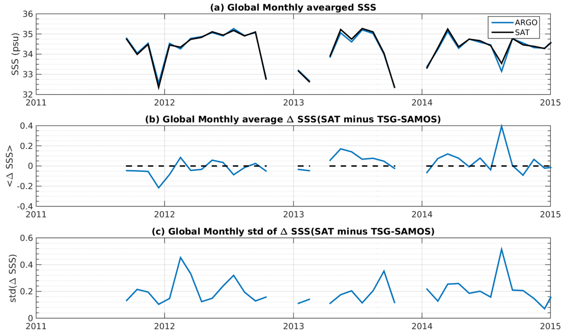
Figure 7: Time series of the monthly averaged mean SSS (top), mean \Delta SSS (Satellite - TSG-SAMOS) and STD of \Delta SSS (Satellite - TSG-SAMOS) over the Pacific Ocean Pi-MEP region considering all match-ups collected by the Pi-MEP platform.
