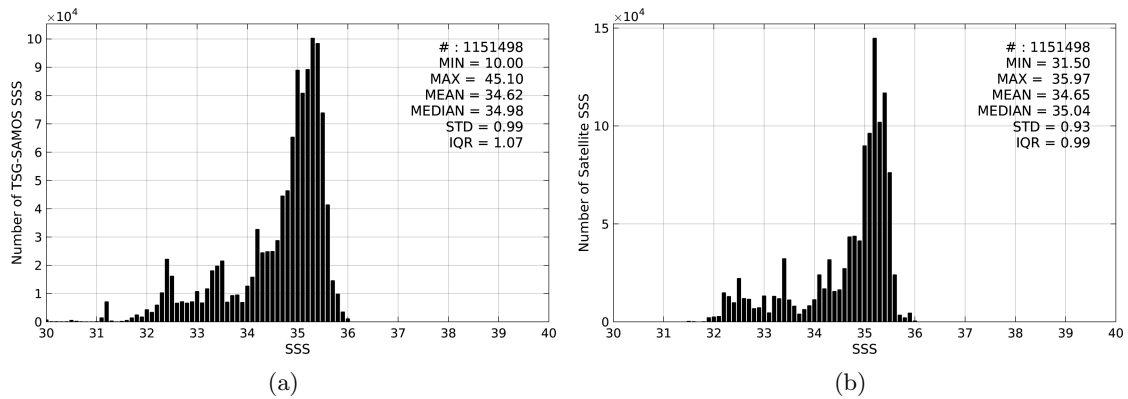
Figure 2: Histograms of SSS from TSG-SAMOS (a) and Aquarius-L4-IPRC-V4-MONTHLY (b) considering all match-up pairs per bins of 0.1 over the Pacific Ocean Pi-MEP region and for the full satellite product period.
