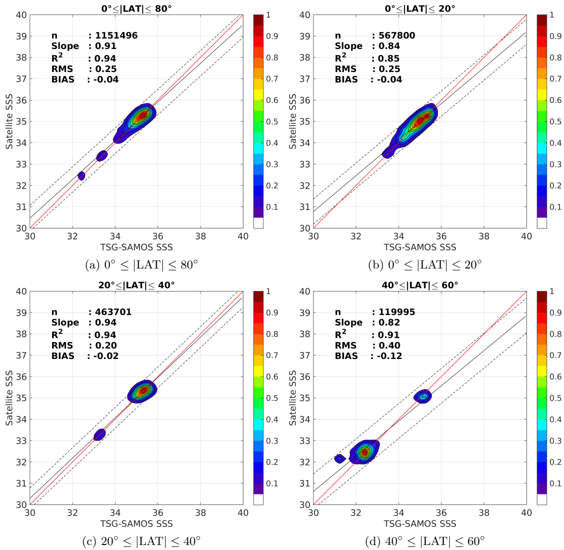
Figure 9: Contour maps of the concentration of Aquarius-L4-IPRC-V4-MONTHLY SSS (y-axis) versus TSG-SAMOS SSS (x-axis) at match-up pairs for different latitude bands. For each plot, the red line shows x=y . The black thin and dashed lines indicate a linear fit through the data cloud and the \pm 95\% confidence levels, respectively. The number match-up pairs n , the slope and R^2 coefficient of the linear fit, the root mean square (RMS) and the mean bias between satellite and in situ data are indicated for each latitude band in each plots.
