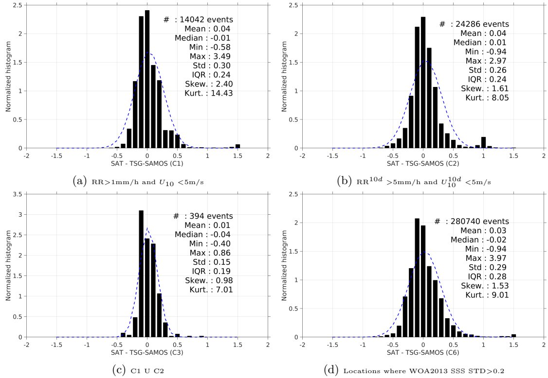
Figure 13: Normalized histogram of \Delta SSS (Aquarius-L4-IPRC-V4-MONTHLY - TSG-SAMOS) for 6 different subdatasets corresponding to: RR > 1mm/h and U_{10} < 5 m/s (a), RR^{10d} > 5 mm/h and U_{10}^{10d} < 5 m/s (b), C1 U C2 (c), Locations where WOA2013 SSS STD > 0.2 (d).
