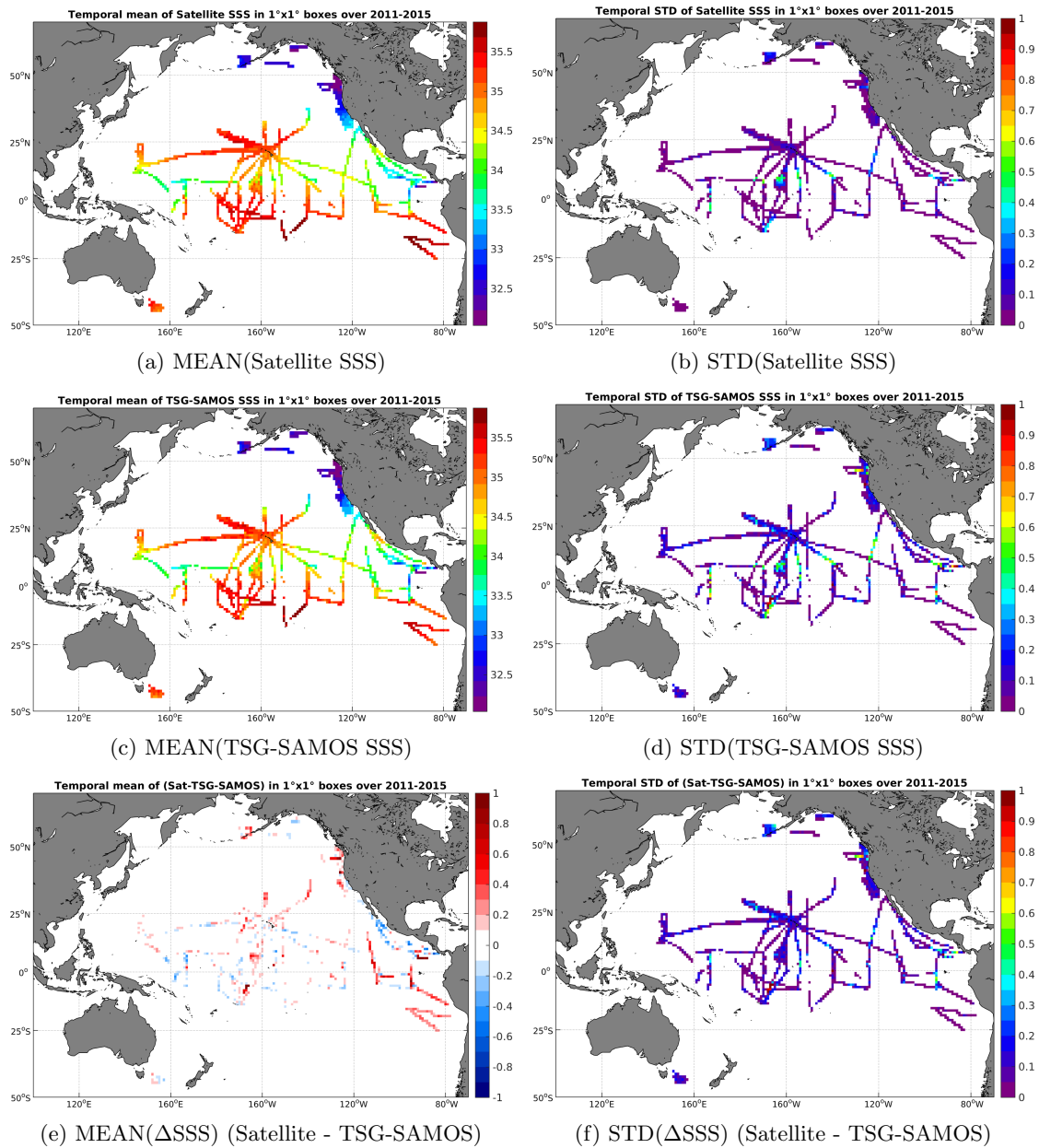
Figure 6: Temporal mean (left) and STD (right) of SSS from Aquarius-L4-IPRC-V4-MONTHLY (top), TSG-SAMOS (middle), and of \Delta SSS (Satellite - TSG-SAMOS). Only match-up pairs are used to generate these maps.
