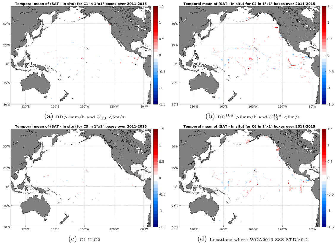
Figure 12: Temporal mean gridded over spatial boxes of size 1^\circ \times 1^\circ of \Delta SSS (Aquarius-L4-IPRC-V4-MONTHLY - TSG-SAMOS) for 4 different subdatasets corresponding to: RR > 1\text{mm/h} and U_{10} < 5\text{m/s} (a), RR^{10d} > 5\text{mm/h} and U_{10}^{10d} < 5\text{m/s} (b), C1 U C2 (c), Locations where WOA2013 SSS STD > 0.2 (d).
