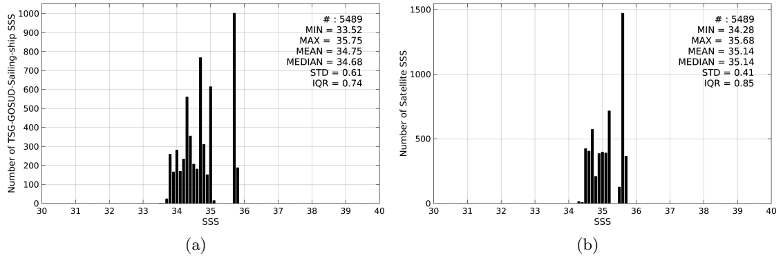
Figure 2: Histograms of SSS from TSG-GOSUD-Sailing-ship (a) and Aquarius-L4-IPRC-V4-MONTHLY (b) considering all match-up pairs per bins of 0.1 over the Pacific Ocean Pi-MEP region and for the full satellite product period.
