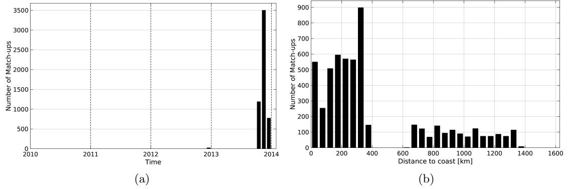
Figure 1: Number of match-ups between TSG-GOSUD-Sailing-ship and Aquarius-L4-IPRC-V4-MONTHLY SSS as a function of time (a) and as function of the distance to coast (b) over the Pacific Ocean Pi-MEP region and for the full satellite product period.
