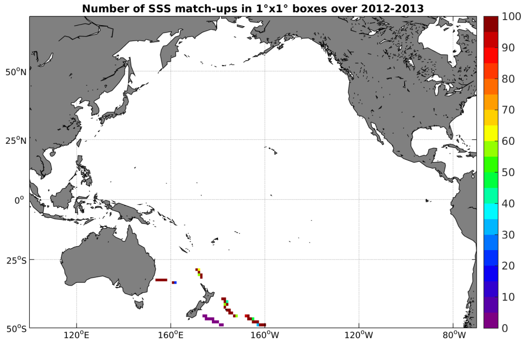
Figure 4: Number of SSS match-ups between TSG-GOSUD-Sailing-ship SSS and the Aquarius-L4-IPRC-V4-MONTHLY SSS product for the Pacific Ocean Pi-MEP region over 1^\circ \times 1^\circ boxes and for the full satellite product period.
