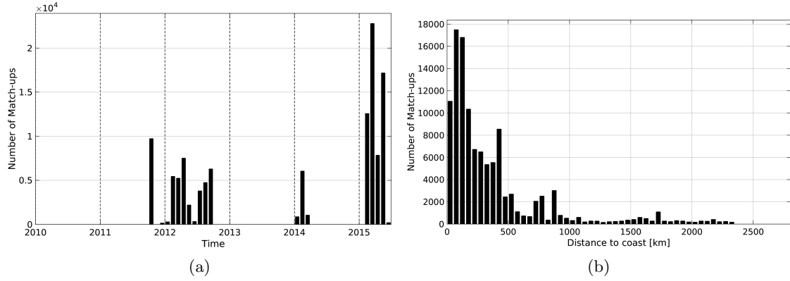
Figure 1: Number of match-ups between TSG-GOSUD-Research-vessel and Aquarius-L4-IPRC-V4-MONTHLY SSS as a function of time (a) and as function of the distance to coast (b) over the Pacific Ocean Pi-MEP region and for the full satellite product period.
