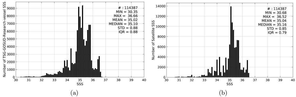
Figure 2: Histograms of SSS from TSG-GOSUD-Research-vessel (a) and Aquarius-L4-IPRC-V4-MONTHLY (b) considering all match-up pairs per bins of 0.1 over the Pacific Ocean Pi-MEP region and for the full satellite product period.
