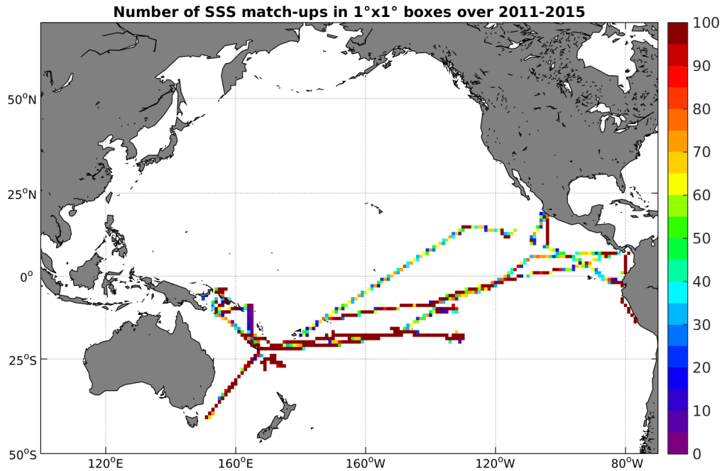
Figure 4: Number of SSS match-ups between TSG-GOSUD-Research-vessel SSS and the Aquarius-L4-IPRC-V4-MONTHLY SSS product for the Pacific Ocean Pi-MEP region over 1^\circ \times 1^\circ boxes and for the full satellite product period.
