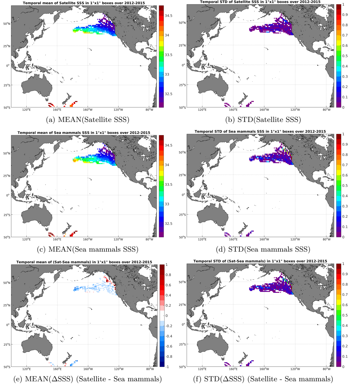
Figure 6: Temporal mean (left) and STD (right) of SSS from Aquarius-L4-IPRC-V4-MONTHLY (top), Sea mammals (middle), and of \Delta SSS (Satellite - Sea mammals). Only match-up pairs are used to generate these maps.
