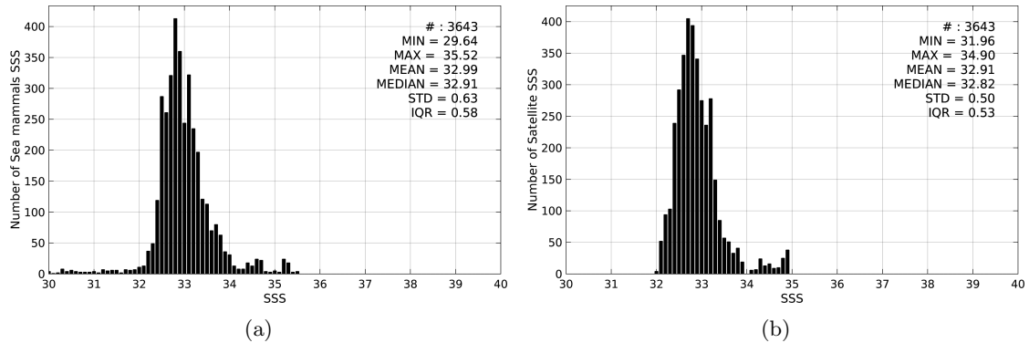
Figure 2: Histograms of SSS from Sea mammals (a) and Aquarius-L4-IPRC-V4-MONTHLY (b) considering all match-up pairs per bins of 0.1 over the Pacific Ocean Pi-MEP region and for the full satellite product period.
