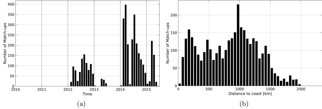
Figure 1: Number of match-ups between Sea mammals and Aquarius-L4-IPRC-V4-MONTHLY SSS as a function of time (a) and as function of the distance to coast (b) over the Pacific Ocean Pi-MEP region and for the full satellite product period.
