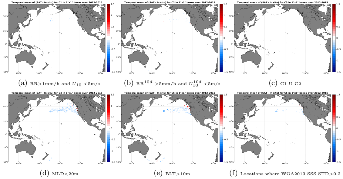
Figure 12: Temporal mean gridded over spatial boxes of size 1^\circ \times 1^\circ of \Delta SSS (Aquarius-L4-IPRC-V4-MONTHLY - Sea mammals) for 6 different subdatasets corresponding to: RR > 1\text{mm/h} and U_{10} < 5\text{m/s} (a), RR^{10d} > 5\text{mm/h} and U_{10}^{10d} < 5\text{m/s} (b), C1 U C2 (c), MLD < 20\text{m} (d), BLT > 10\text{m} (e), Locations where WOA2013 SSS STD > 0.2 (f).
