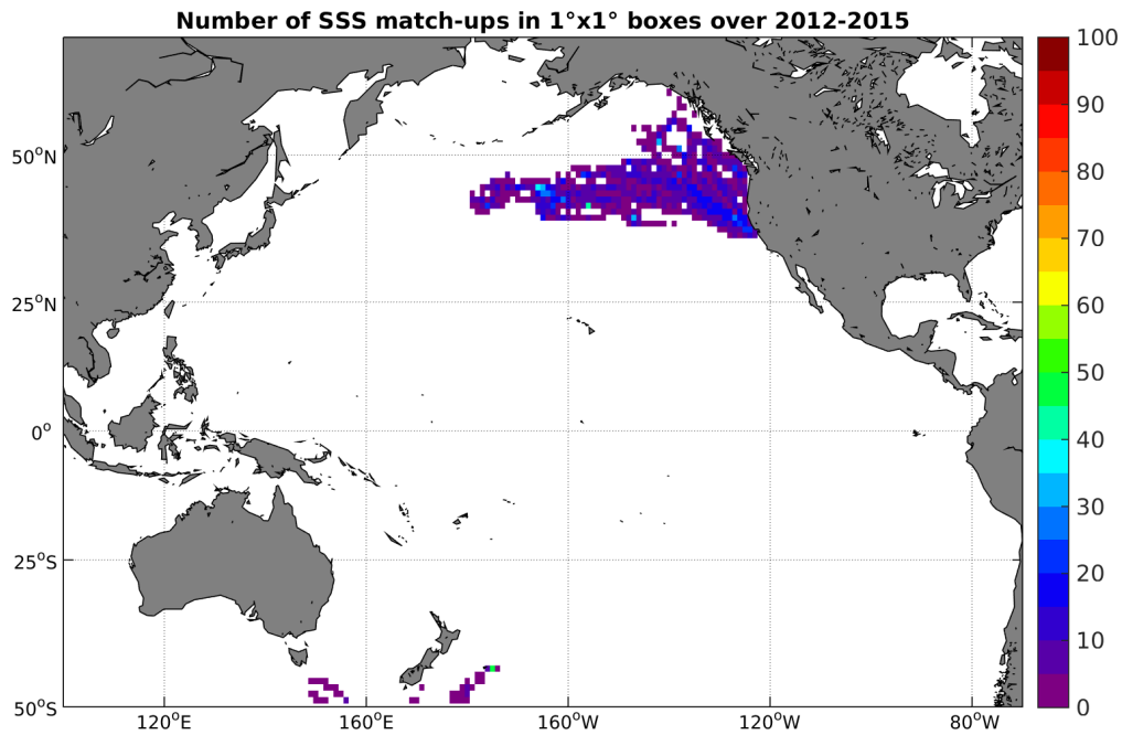
Figure 4: Number of SSS match-ups between Sea mammals SSS and the Aquarius-L4-IPRC-V4-MONTHLY SSS product for the Pacific Ocean Pi-MEP region over 1^\circ \times 1^\circ boxes and for the full satellite product period.
