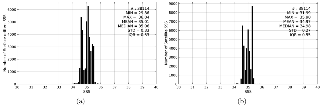
Figure 2: Histograms of SSS from Surface drifters (a) and Aquarius-L4-IPRC-V4-MONTHLY (b) considering all match-up pairs per bins of 0.1 over the Pacific Ocean Pi-MEP region and for the full satellite product period.
