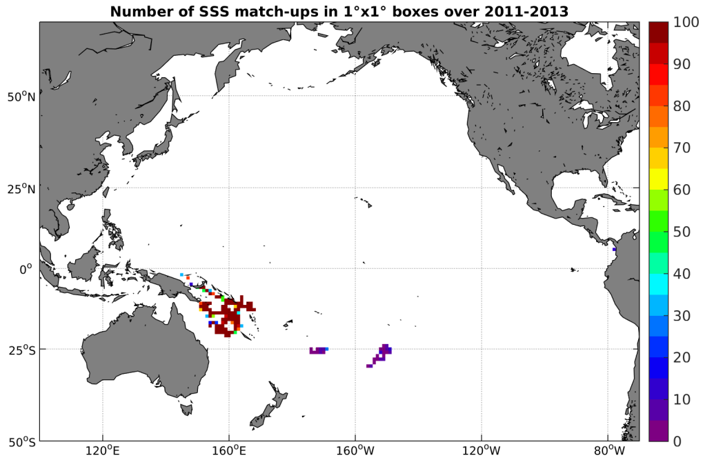
Figure 3: Number of SSS match-ups between Surface drifters SSS and the Aquarius-L4-IPRC-V4-MONTHLY SSS product for the Pacific Ocean Pi-MEP region over 1^\circ \times 1^\circ boxes and for the full satellite product period.
