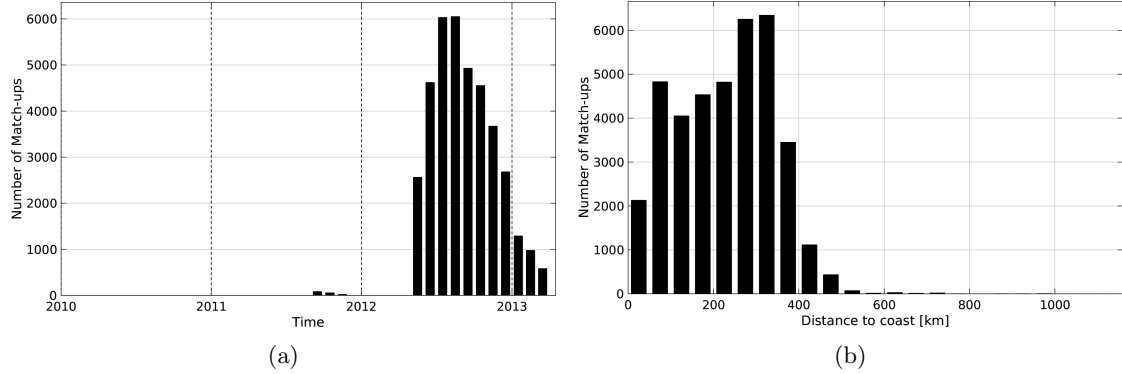
Figure 1: Number of match-ups between Surface drifters and Aquarius-L4-IPRC-V4-MONTHLY SSS as a function of time (a) and as function of the distance to coast (b) over the Pacific Ocean Pi-MEP region and for the full satellite product period.
