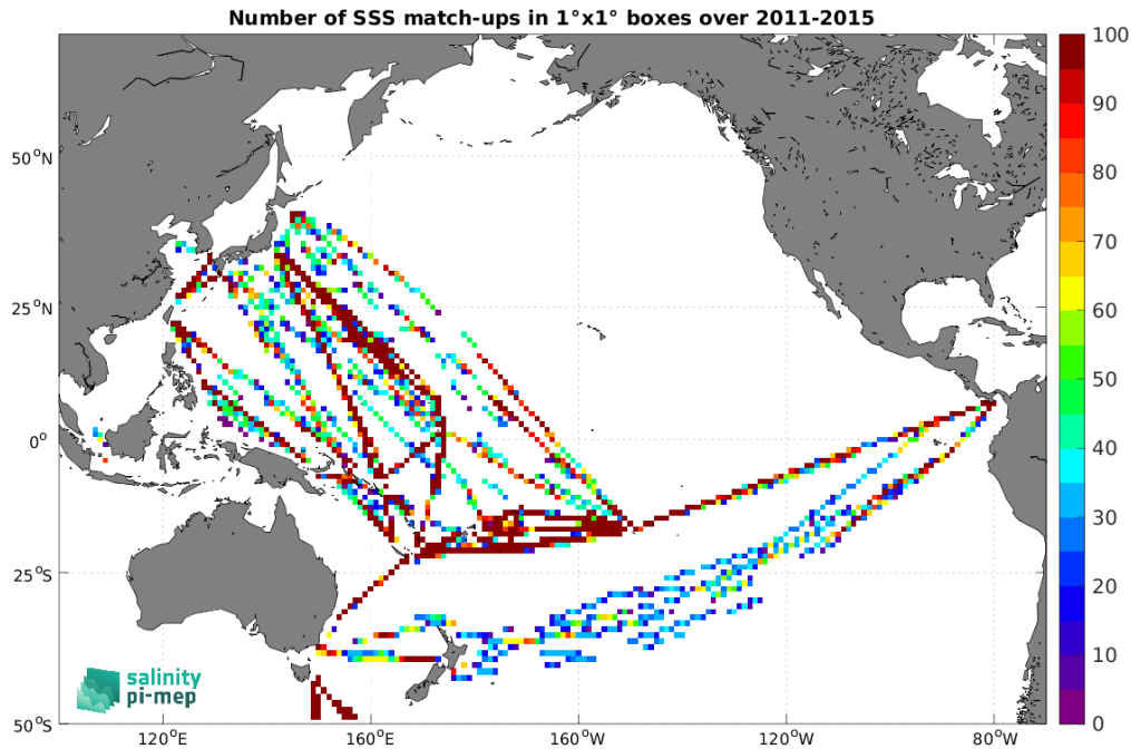
Figure 5: Number of SSS match-ups between TSG (LEGOS-DM) SSS and the Aquarius SSS L3 OR v5 - 7-Day running (NASA-GSFC) SSS product for the Pacific Ocean Pi-MEP region over 1^\circ \times 1^\circ boxes and for the full satellite product period.
