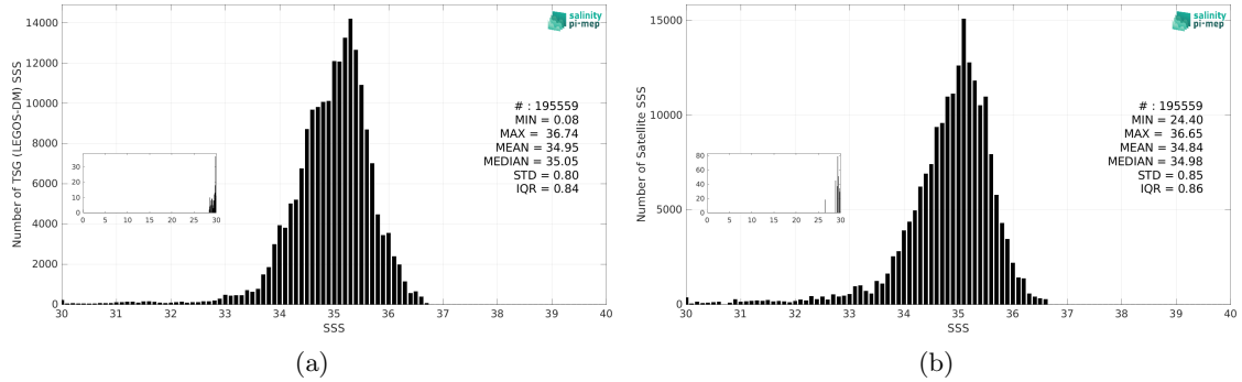
Figure 3: Histograms of SSS from TSG (LEGOS-DM) (a) and Aquarius SSS L3 OR v5 - 7-Day running (NASA-GSFC) (b) considering all match-up pairs per bins of 0.1 over the Pacific Ocean Pi-MEP region and for the full satellite product period.
