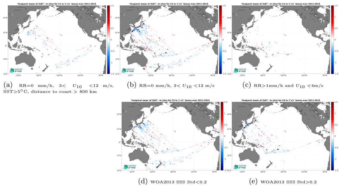
Figure 14: Temporal mean gridded over spatial boxes of size 1^\circ \times 1^\circ of \Delta\text{SSS} (Aquarius SSS L3 OR v5 - 7-Day running (NASA-GSFC) - TSG (LEGOS-DM)) for 5 different subdatasets corresponding to:RR=0 mm/h, 3 < U_{10} < 12 m/s, SST >5^\circ\text{C} , distance to coast > 800 km (a), RR=0 mm/h, 3 < U_{10} < 12 m/s (b), RR >1 mm/h and U_{10} < 4 m/s (c), WOA2013 SSS Std <0.2 (d), WOA2013 SSS Std >0.2 (e).
