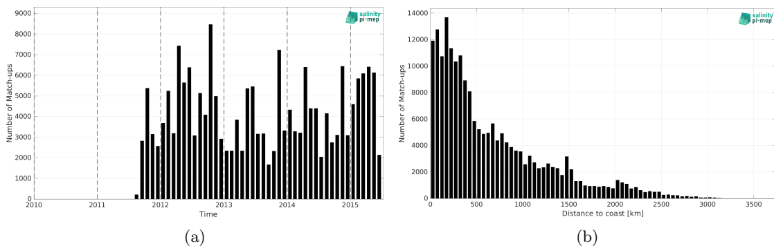
Figure 2: Number of match-ups between TSG (LEGOS-DM) and Aquarius SSS L3 OR v5 - 7-Day running (NASA-GSFC) SSS as a function of time (a) and as function of the distance to coast (b) over the Pacific Ocean Pi-MEP region and for the full satellite product period.
