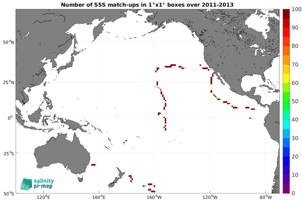
Figure 5: Number of SSS match-ups between TSG (GOSUD-Sailing-ship) SSS and the Aquarius SSS L3 OR v5 - 7-Day running (NASA-GSFC) SSS product for the Pacific Ocean Pi-MEP region over 1^\circ \times 1^\circ boxes and for the full satellite product period.
