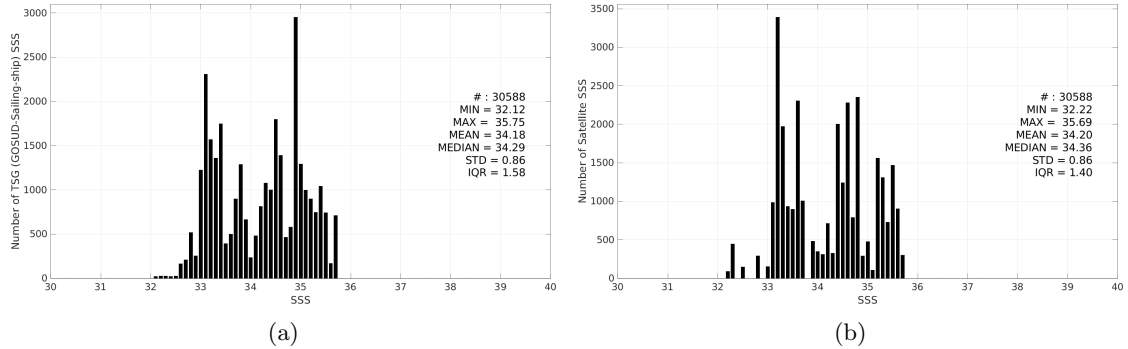
Figure 3: Histograms of SSS from TSG (GOSUD-Sailing-ship) (a) and Aquarius SSS L3 OR v5 - 7-Day running (NASA-GSFC) (b) considering all match-up pairs per bins of 0.1 over the Pacific Ocean Pi-MEP region and for the full satellite product period.
