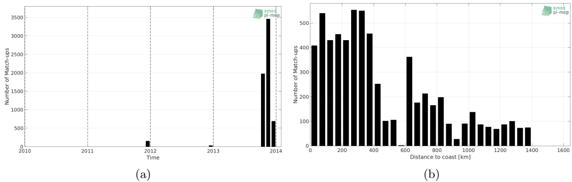
Figure 1: Number of match-ups between TSG-GOSUD-Sailing-ship and Aquarius-L3-OR-V5-7DAY-RUNNING-1DEG SSS as a function of time (a) and as function of the distance to coast (b) over the Pacific Ocean Pi-MEP region and for the full satellite product period.
