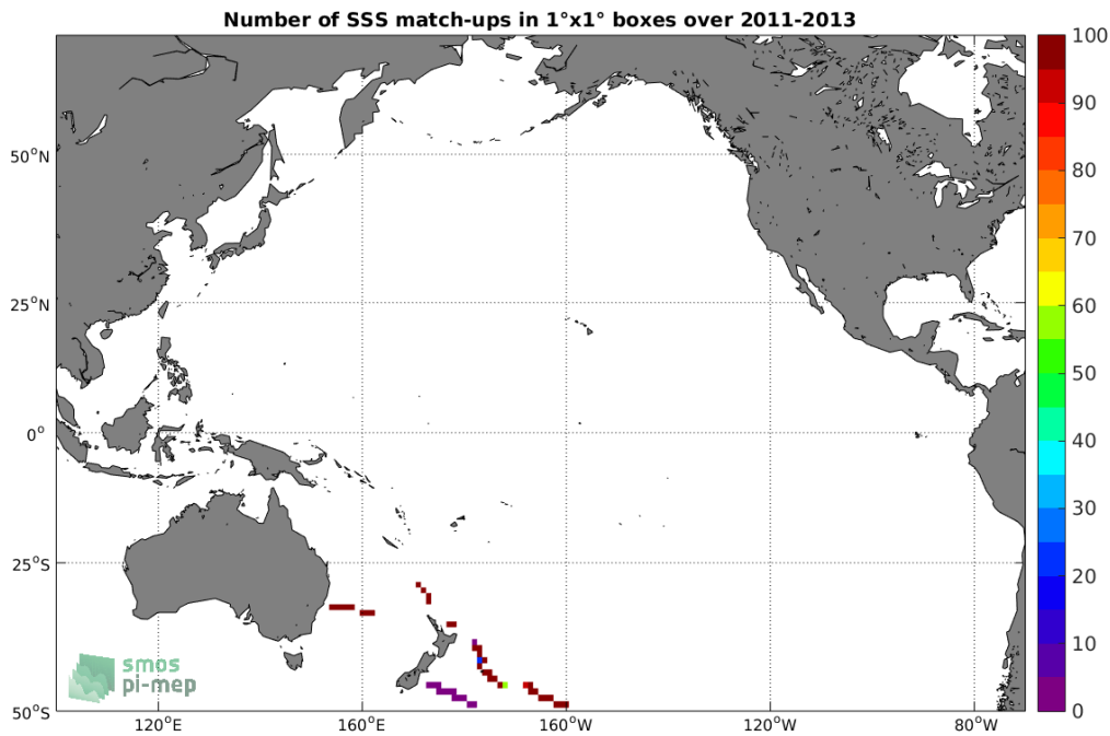
Figure 4: Number of SSS match-ups between TSG-GOSUD-Sailing-ship SSS and the Aquarius-L3-OR-V5-7DAY-RUNNING-1DEG SSS product for the Pacific Ocean Pi-MEP region over 1°x1° boxes and for the full satellite product period.
