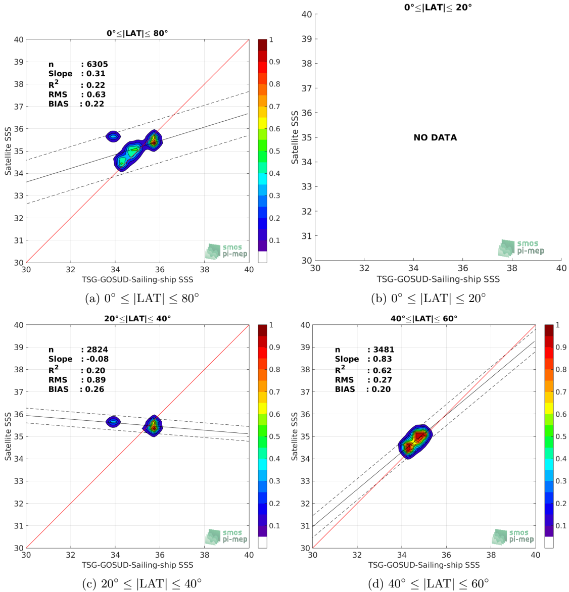
Figure 9: Contour maps of the concentration of Aquarius-L3-OR-V5-7DAY-RUNNING-1DEG SSS (y-axis) versus TSG-GOSUD-Sailing-ship SSS (x-axis) at match-up pairs for different latitude bands. For each plot, the red line shows x=y . The black thin and dashed lines indicate a linear fit through the data cloud and the \pm 95\% confidence levels, respectively. The number of match-up pairs n , the slope and R^2 coefficient of the linear fit, the root mean square (RMS) and the mean bias between satellite and in situ data are indicated for each latitude band in each plot.
