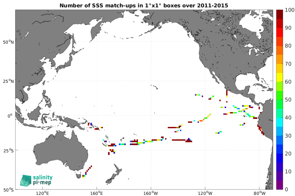
Figure 5: Number of SSS match-ups between TSG (GOSUD-Research-vessel) SSS and the Aquarius SSS L3 OR v5 - 7-Day running (NASA-GSFC) SSS product for the Pacific Ocean Pi-MEP region over 1^\circ \times 1^\circ boxes and for the full satellite product period.
