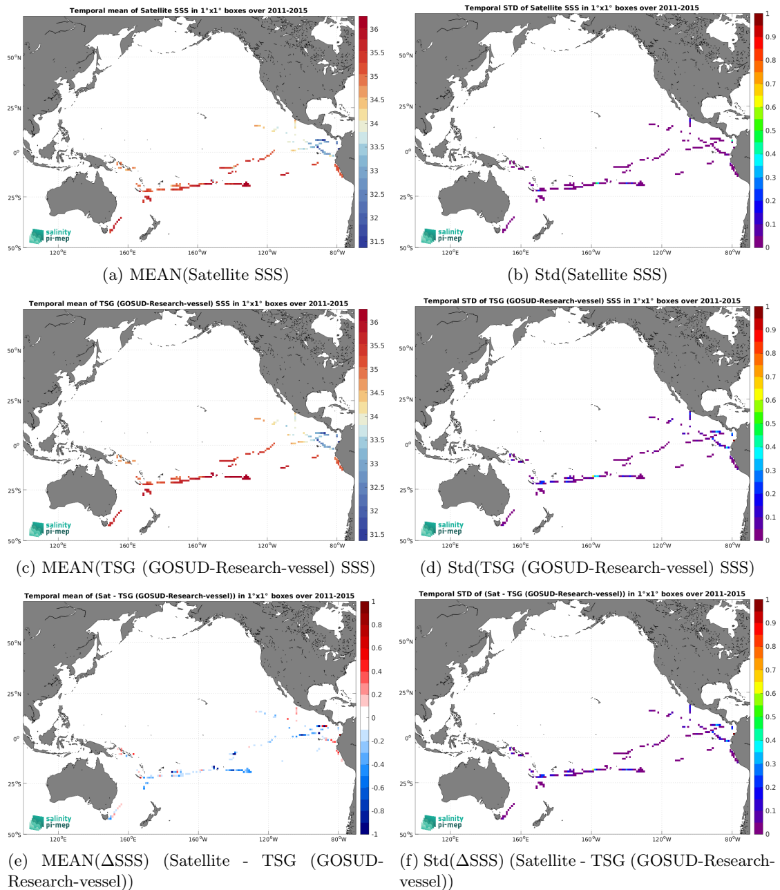
Figure 7: Temporal mean (left) and Std (right) of SSS from Aquarius SSS L3 OR v5 - 7-Day running (NASA-GSFC) (top), TSG (GOSUD-Research-vessel) (middle), and of \Delta SSS (Satellite - TSG (GOSUD-Research-vessel)). Only match-up pairs are used to generate these maps.
