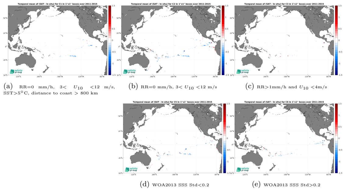
Figure 14: Temporal mean gridded over spatial boxes of size 1^\circ \times 1^\circ of \Delta SSS (Aquarius SSS L3 OR v5 - 7-Day running (NASA-GSFC) - TSG (GOSUD-Research-vessel)) for 5 different subdatasets corresponding to:RR=0 mm/h, 3 < U_{10} < 12 m/s, SST >5^\circ\text{C} , distance to coast > 800 km (a), RR=0 mm/h, 3 < U_{10} < 12 m/s (b), RR >1 mm/h and U_{10} < 4 m/s (c), WOA2013 SSS Std <0.2 (d), WOA2013 SSS Std >0.2 (e).
