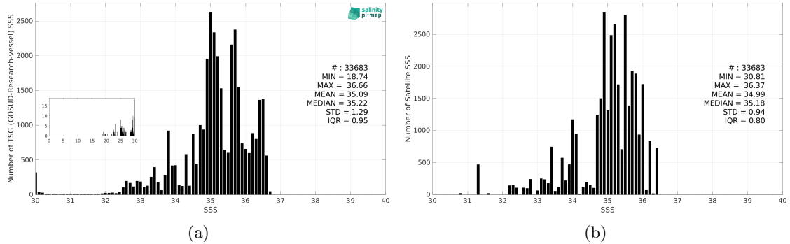
Figure 3: Histograms of SSS from TSG (GOSUD-Research-vessel) (a) and Aquarius SSS L3 OR v5 - 7-Day running (NASA-GSFC) (b) considering all match-up pairs per bins of 0.1 over the Pacific Ocean Pi-MEP region and for the full satellite product period.
