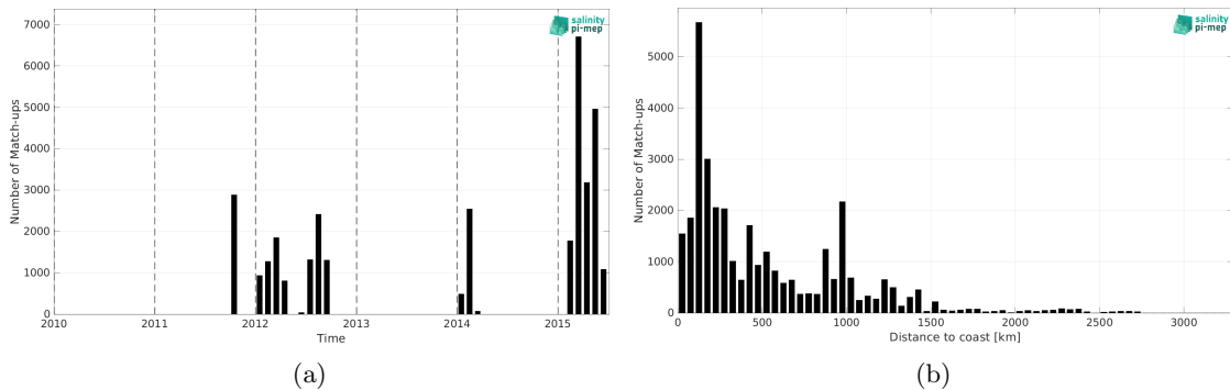
Figure 2: Number of match-ups between TSG (GOSUD-Research-vessel) and Aquarius SSS L3 OR v5 - 7-Day running (NASA-GSFC) SSS as a function of time (a) and as function of the distance to coast (b) over the Pacific Ocean Pi-MEP region and for the full satellite product period.
